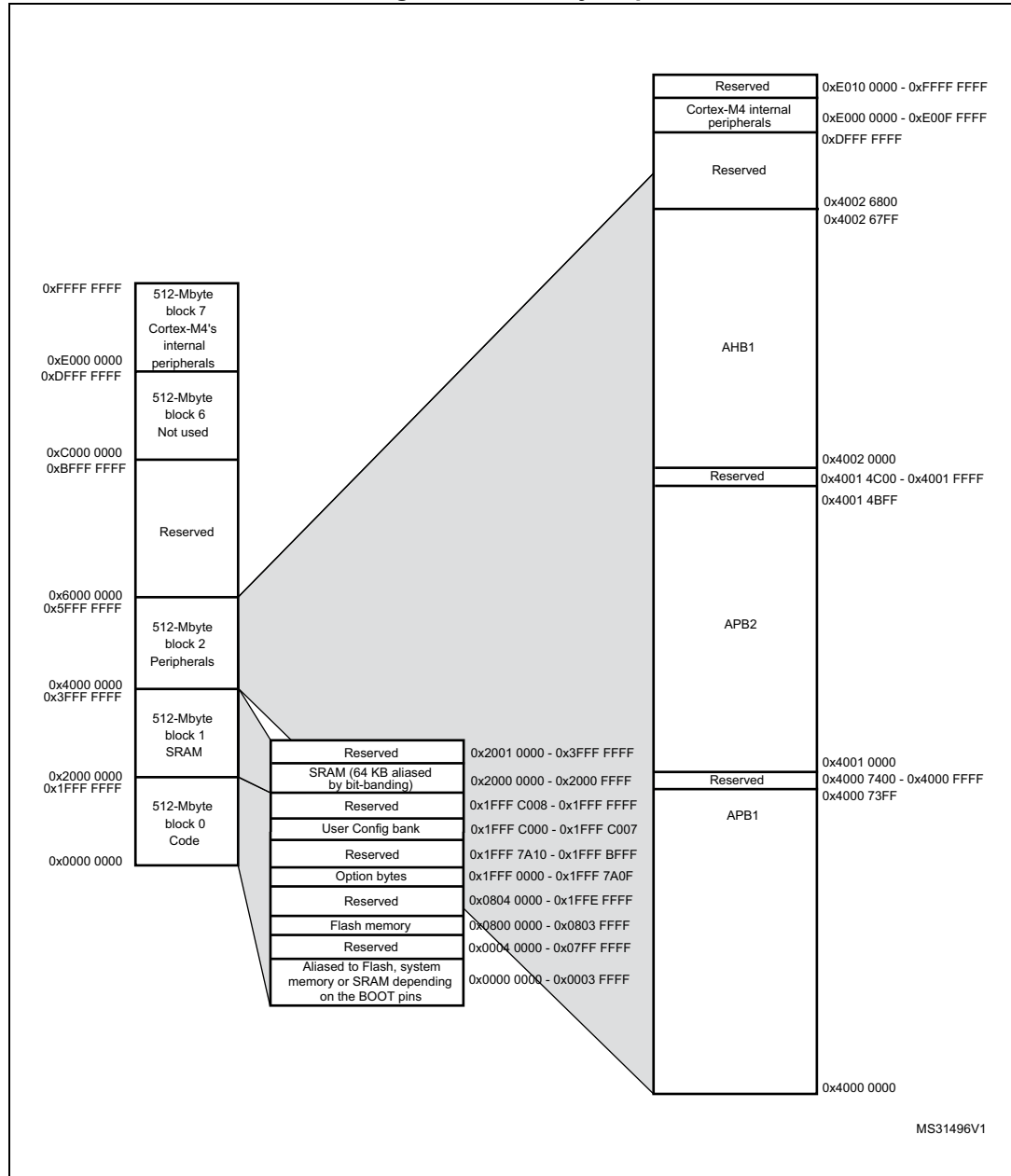
Figure 15. Memory map
