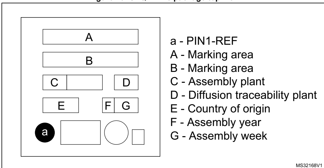
Figure 49. UFQFPN48 package top view
