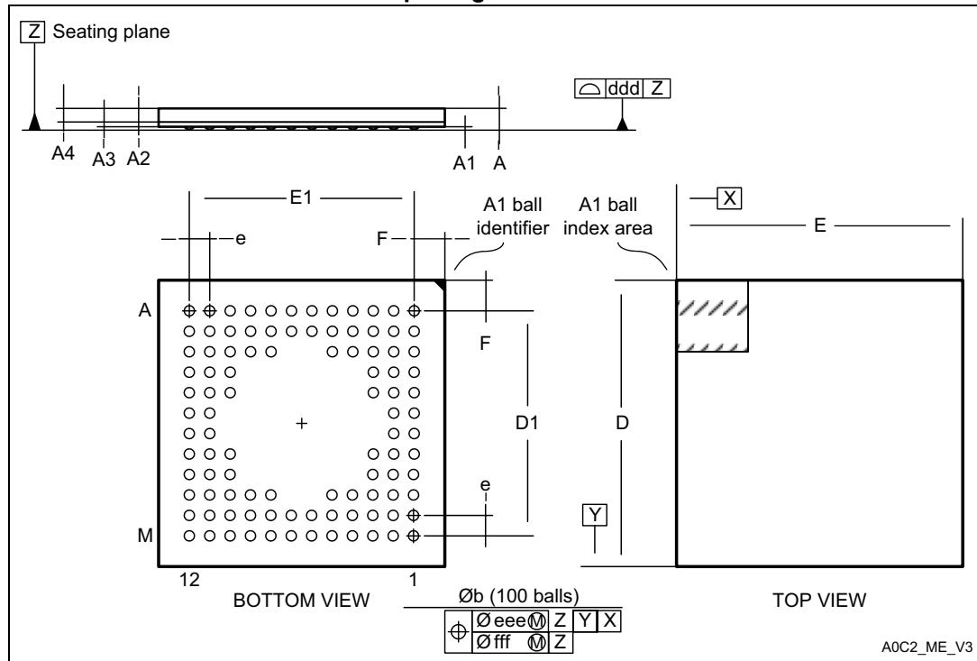
Figure 57. Recommended PCB design rules for pads (0.5 mm-pitch BGA)
