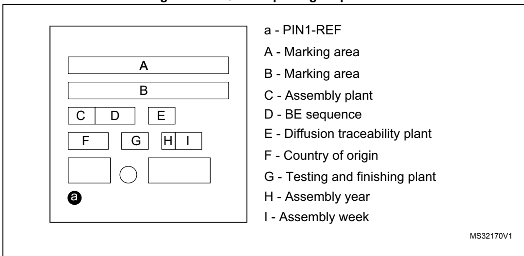
Figure 55. LQFP100 package top view
