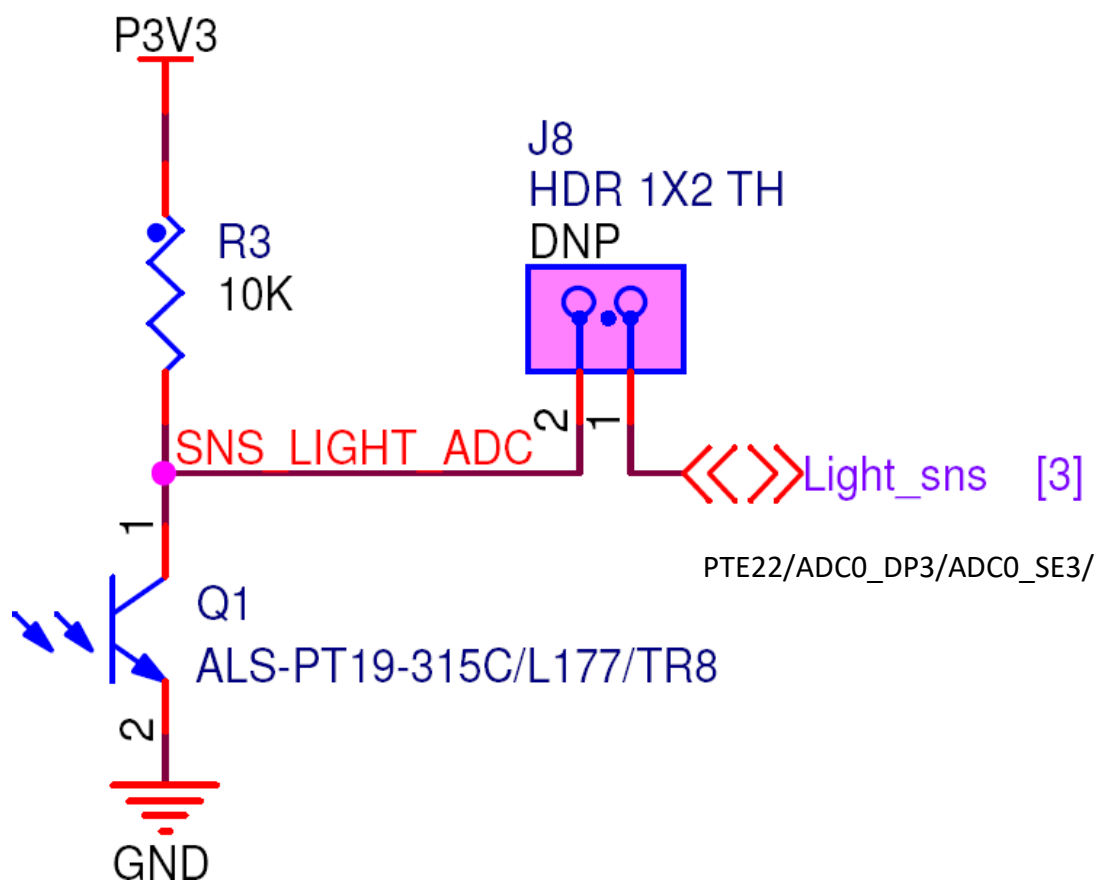
Figure 7 Visible light sensor schematic
