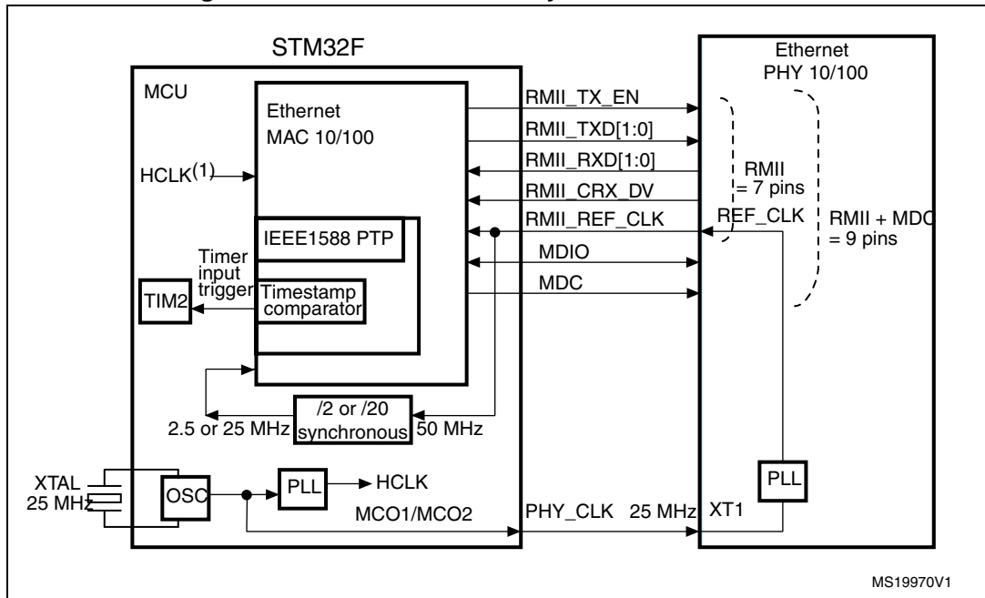
Figure 96. RMIi with a 25 MHz crystal and PHY with PLL
