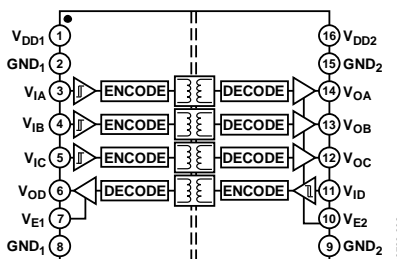
Figure 2. ADuM1401
