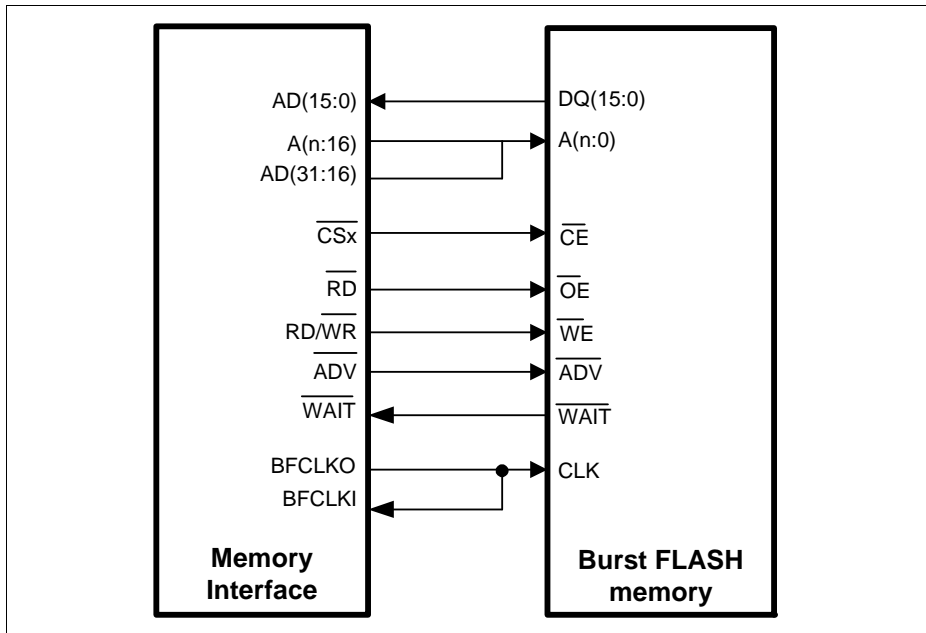
Figure 14-23 Typical Burst Flash Connection
