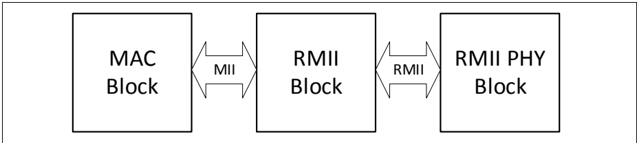
Figure 15-18 RMII Block Diagram
