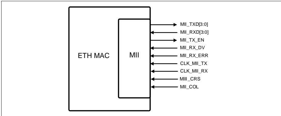
Figure 15-17 Media Independent Interface
