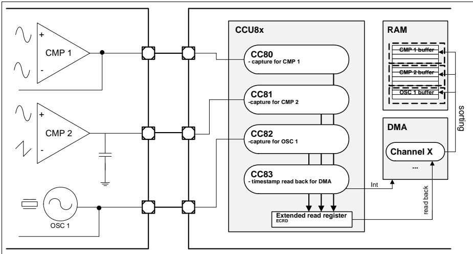
Figure 23-82 Extended read usage scheme example
