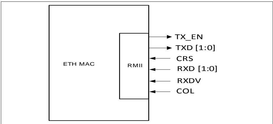
Figure 15-19 RMII Pinout
