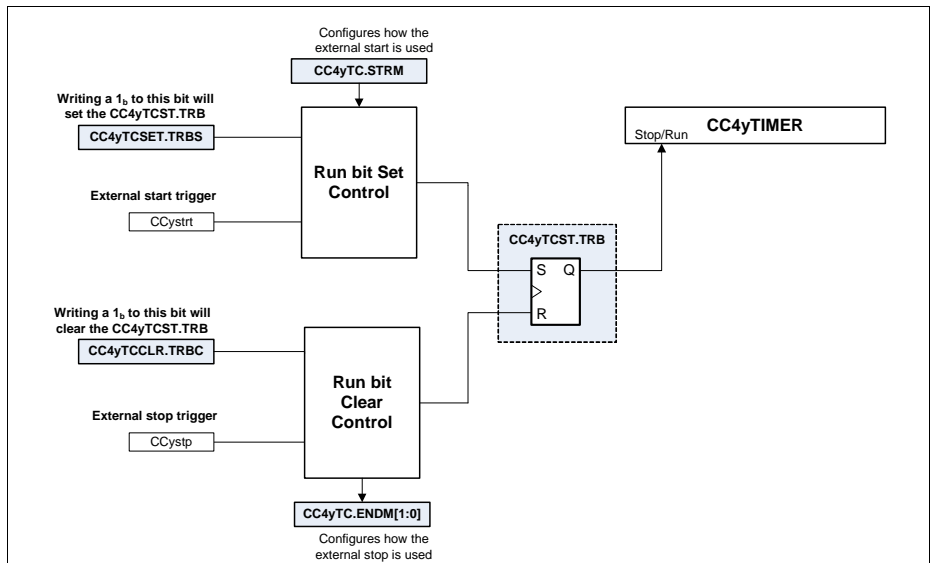
Figure 22-5 Timer start/stop control diagram
