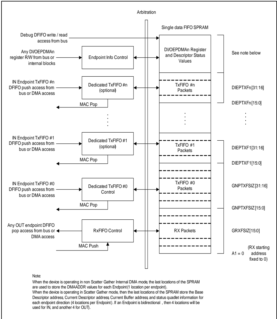
Figure 16-69 Device Mode FIFO Address Mapping
