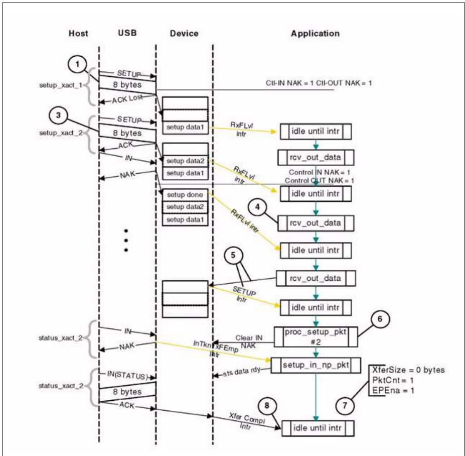
Figure 16-22 Two-Stage Control Transfer
