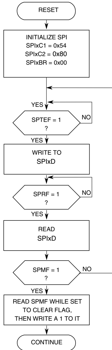
Figure 34-26. Initialization Flowchart Example for SPI Master Device
