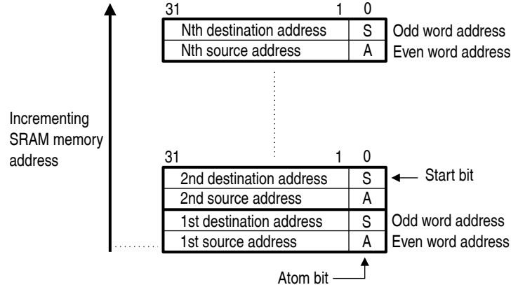
Figure 19-2. MTB execution trace storage format
