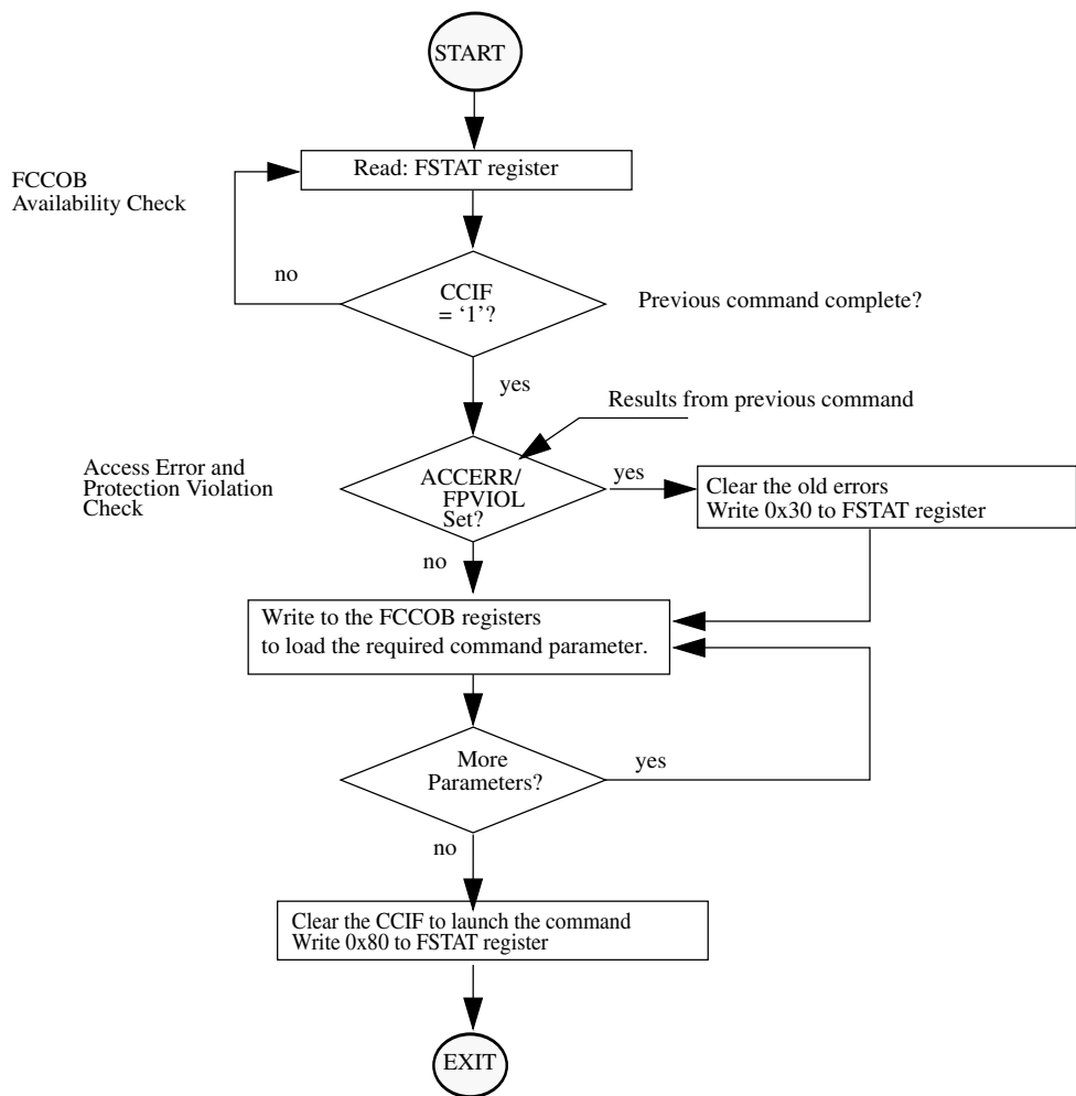
Figure 27-25. Generic Flash Command Write Sequence Flowchart
