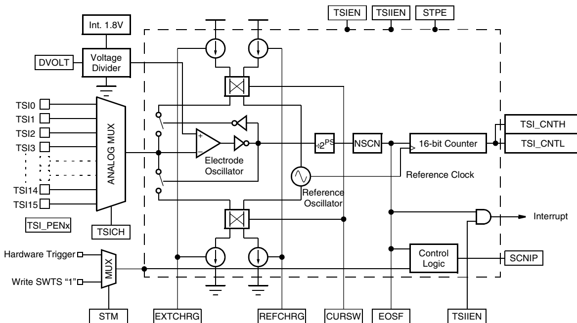
Figure 40-1. TSI module block diagram
