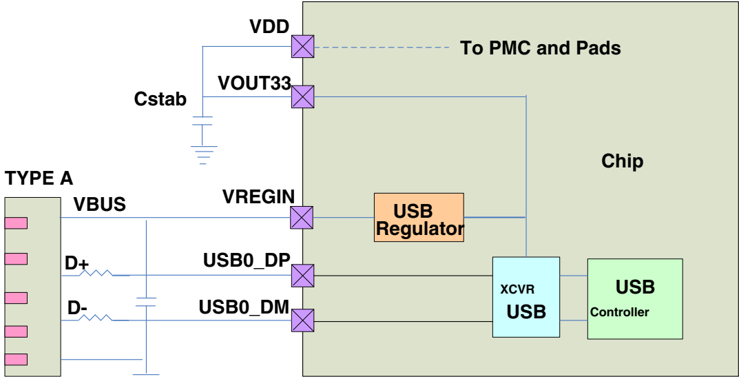
Figure 3-31. USB regulator bus supply
