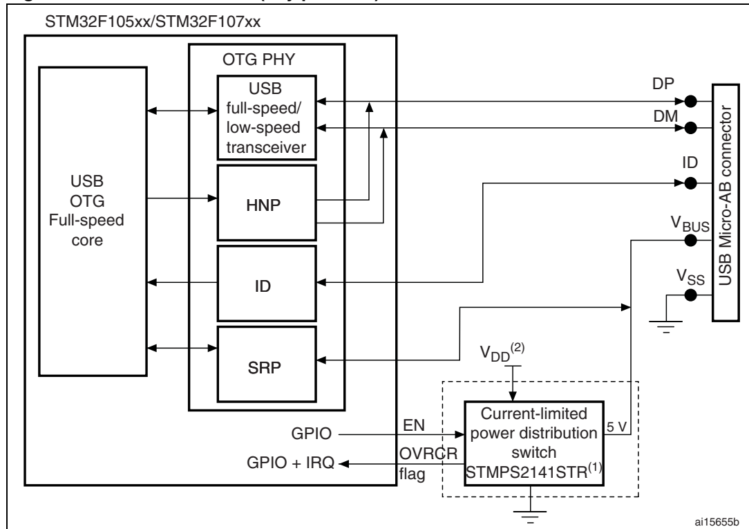
Figure 39. OTG connection (any protocol)
