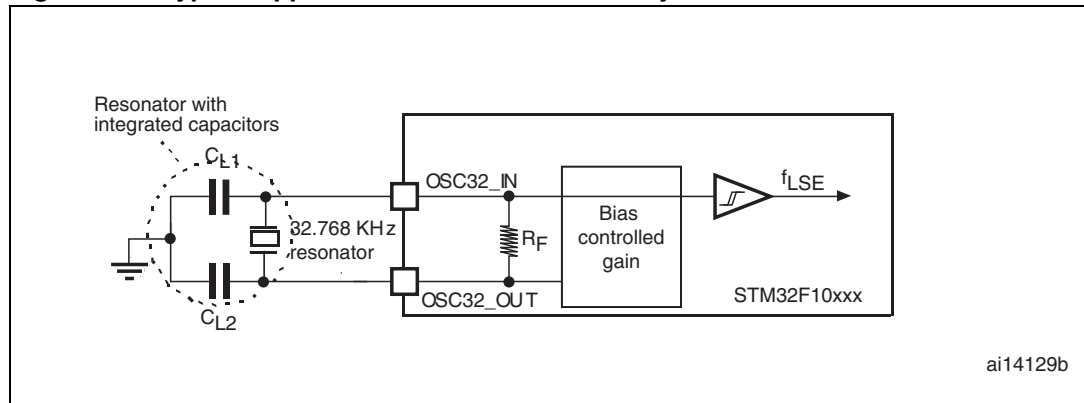
Figure 15. Typical application with a 32.768 kHz crystal
