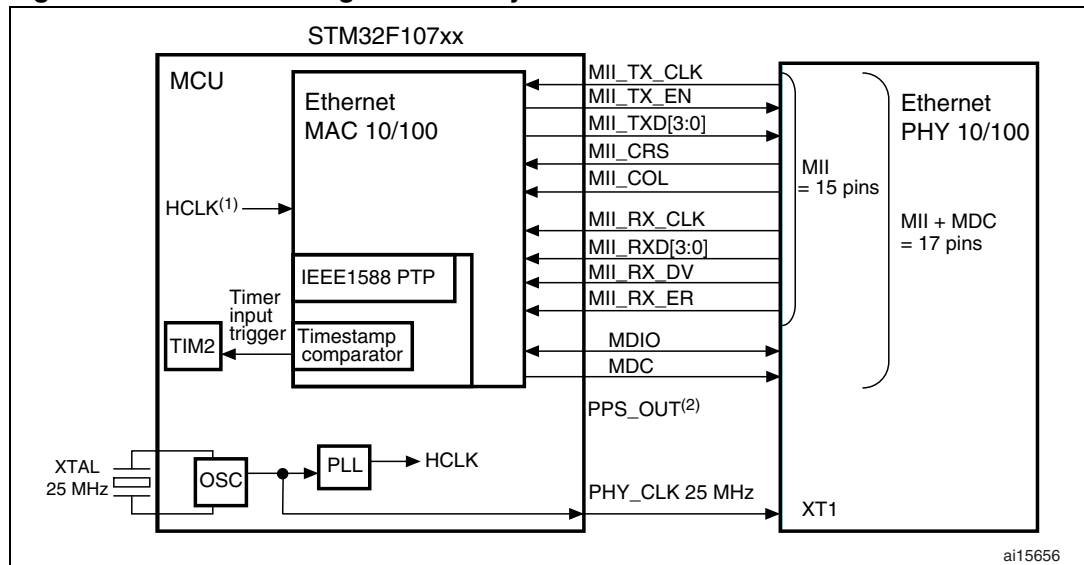
Figure 40. MII mode using a 25 MHz crystal
