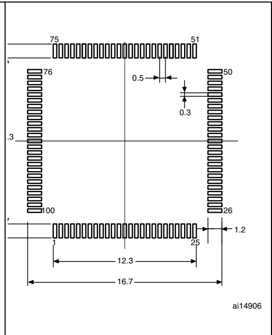
Figure 33. Recommended footprint (1)(2)
