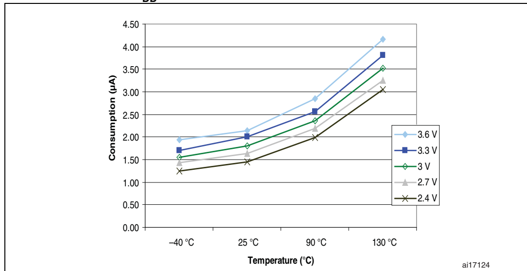
Figure 11. Typical current consumption in Standby mode versus temperature at different V DD values
