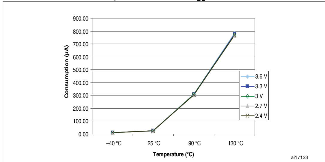
Figure 10. Typical current consumption in Stop mode with regulator in Low-power mode versus temperature at different V DD values
