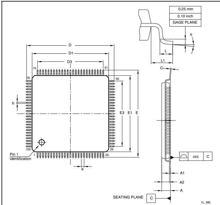
Figure 32. LQFP100, 100-pin low-profile quad flat package outline (1)
