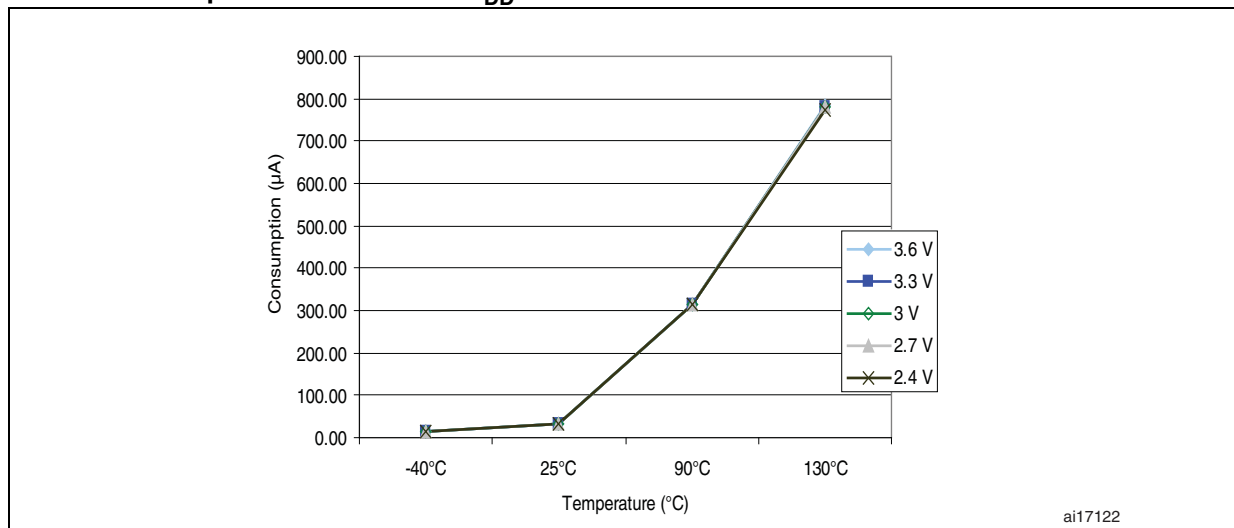
Figure 9. Typical current consumption in Stop mode with regulator in Run mode versus temperature at different V DD values
