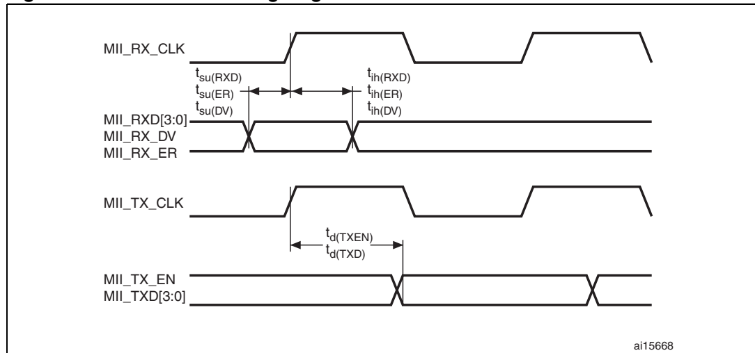
Figure 27. Ethernet MII timing diagram
