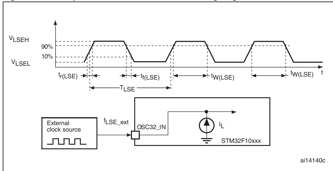
Figure 13. Low-speed external clock source AC timing diagram
