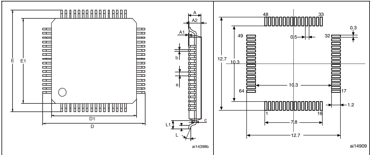
Figure 34. LQFP64 – 64 pin low-profile quad flat package outline (1)
