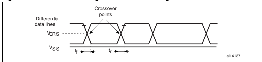
Figure 24. USB OTG FS timings: definition of data signal rise and fall time
