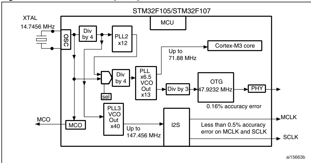
Figure 47. USB OTG FS + I 2 S (Audio) solution
