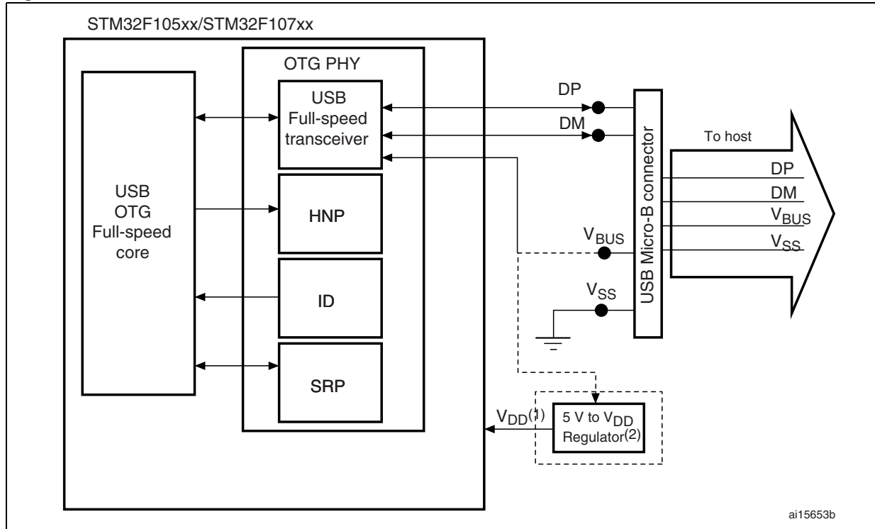
Figure 37. USB OTG FS device mode
