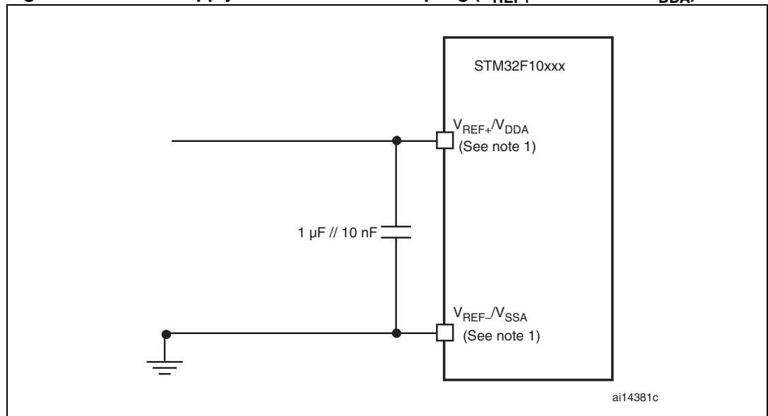
Figure 31. Power supply and reference decoupling ( V_{REF+} connected to V_{DDA} )
