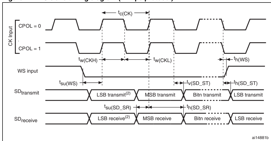
Figure 22. I 2 S slave timing diagram (Philips protocol) (1)
