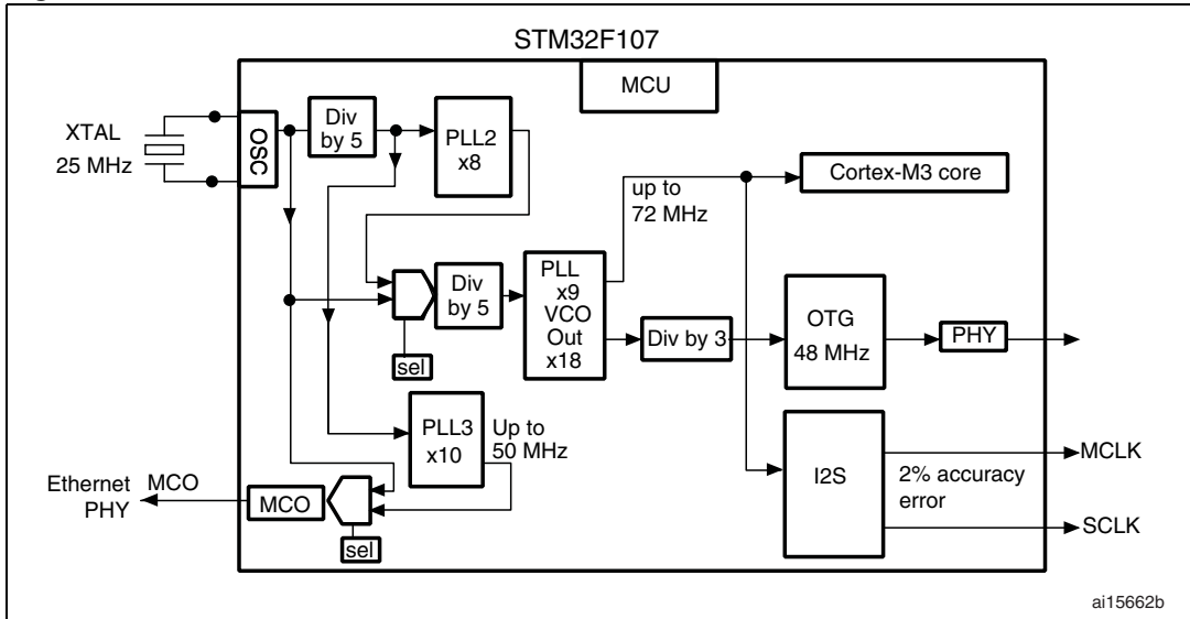
Figure 46. USB OTG FS + Ethernet solution
