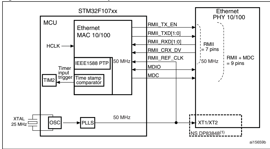
Figure 43. RMIi with a 25 MHz crystal
