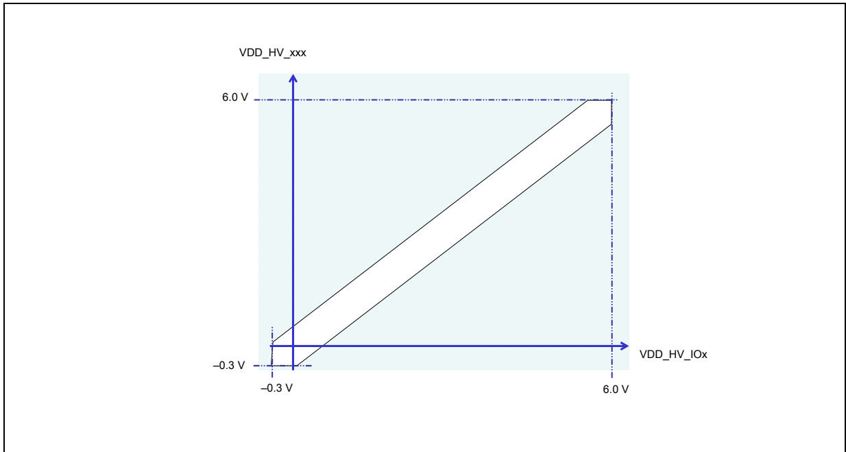
Figure 5. Power supplies constraints ( -0.3\text{ V} \leq V_{DD\_HV\_IOx} \leq 6.0\text{ V} )
