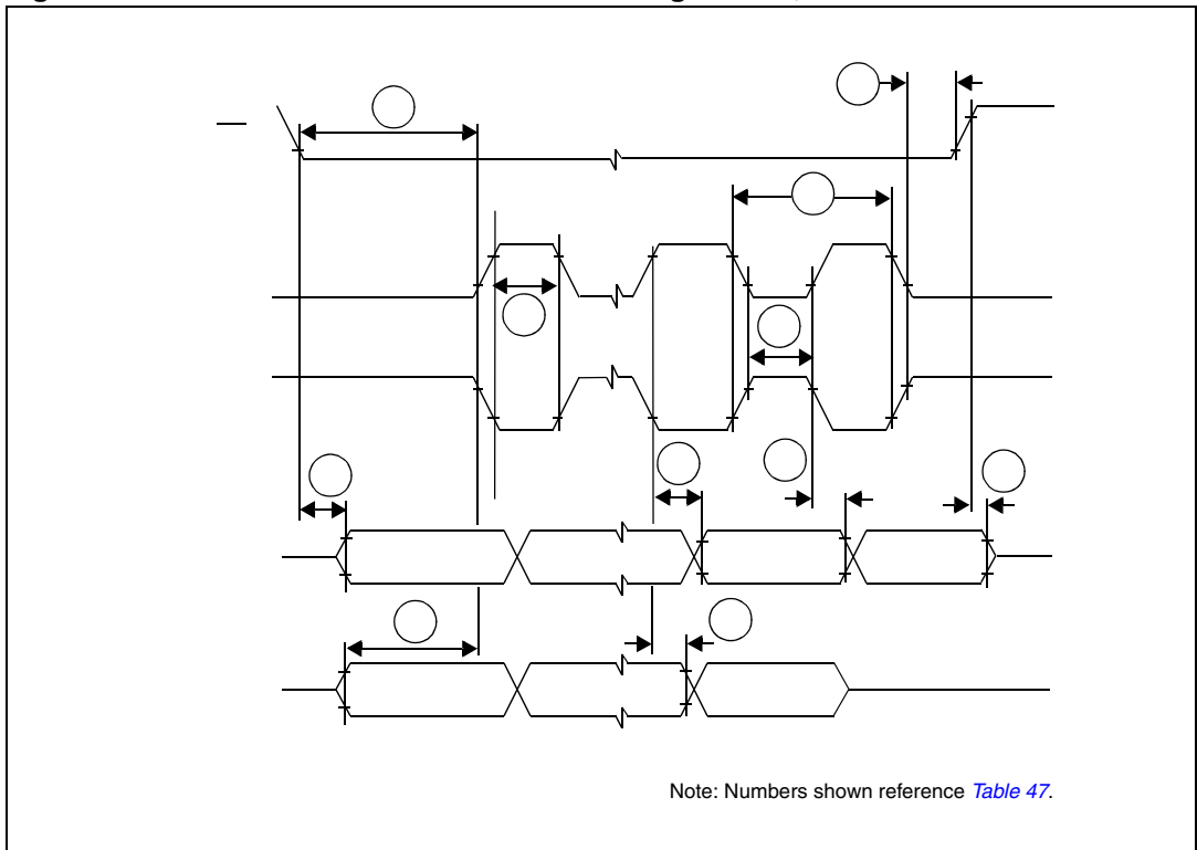
Figure 29. DSPI modified transfer format timing – slave, CPHA = 0
