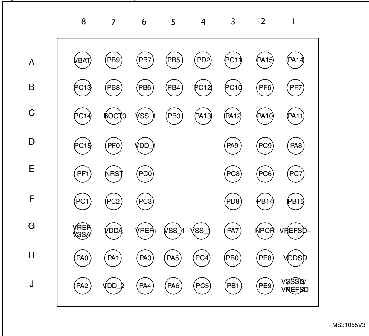
Figure 6. STM32F38x WLCSP66 pinout
