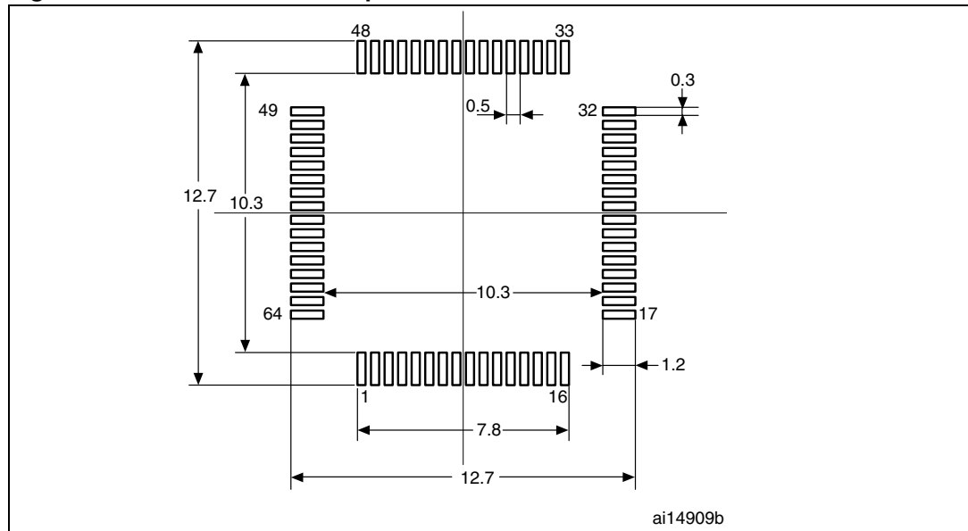
Figure 35. Recommended footprint
