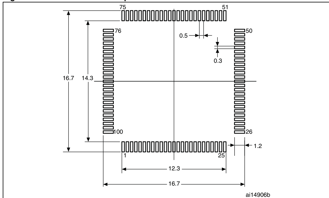
Figure 33. Recommended footprint
