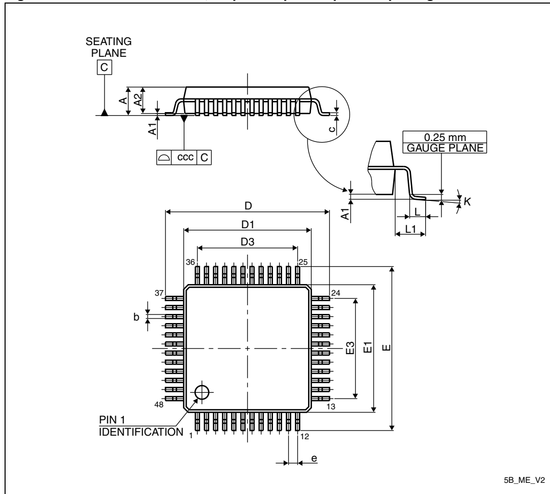
Figure 36. LQFP48 – 7 x 7 mm, 48-pin low-profile quad flat package outline
