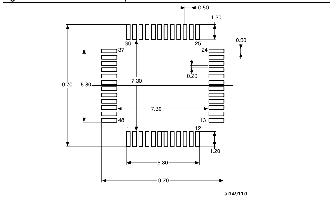
Figure 37. Recommended footprint
