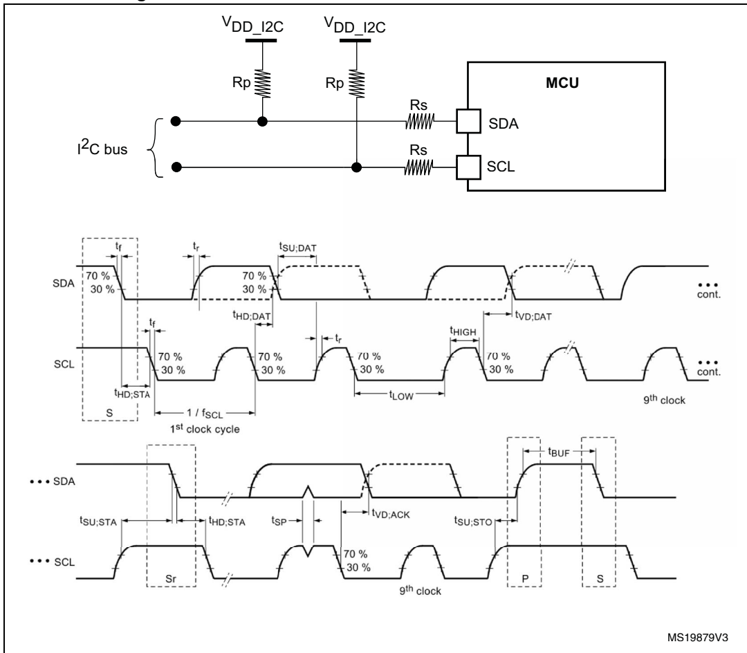
Figure 21. I2C bus AC waveforms and measurement circuit
