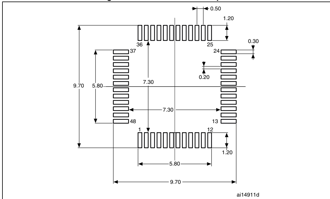
Figure 36. Recommended footprint
