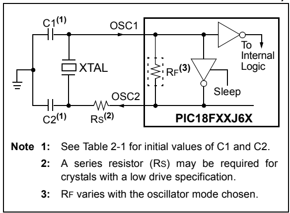
FIGURE 2-2: CRYSTAL OSCILLATOR OPERATION (HS OR HSPLL CONFIGURATION)
