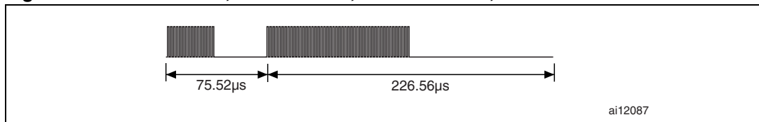
Figure 44. End of frame, low data rate, one subcarrier, Fast commands
