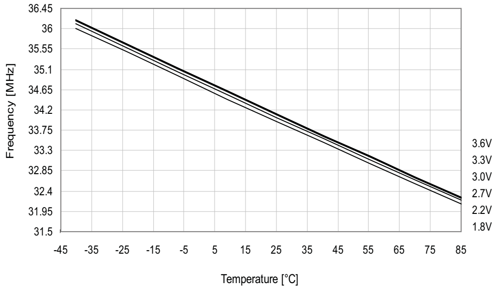
Figure 33-151. 32MHz internal oscillator frequency vs. temperature. DFLL enabled, from the 32.768kHz internal oscillator.
