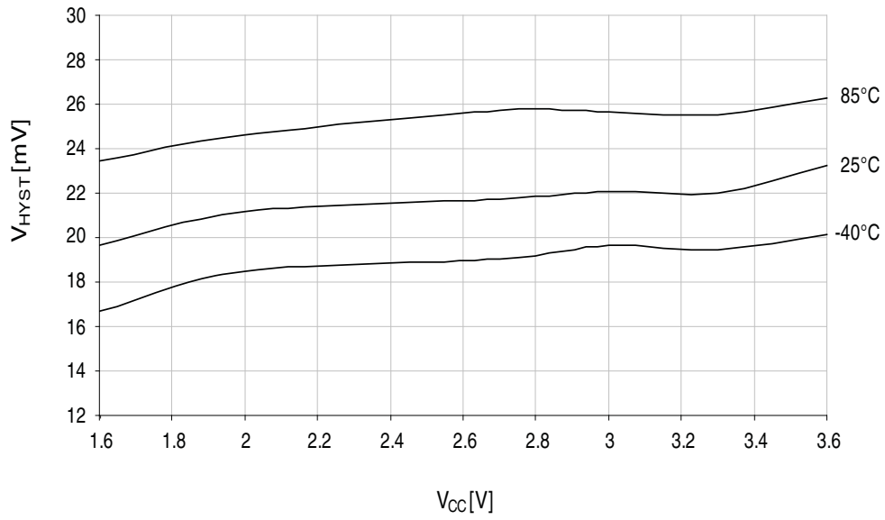
Figure 33-50. Analog comparator hysteresis vs. V_{CC} .
