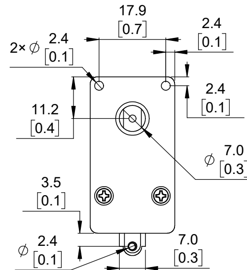
④ Front view Scale 1:1
