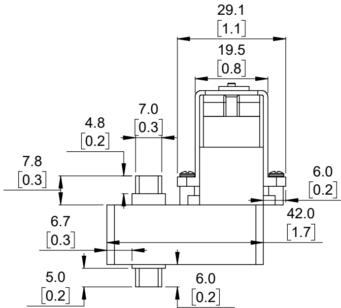
③ Top view Scale 1:1
