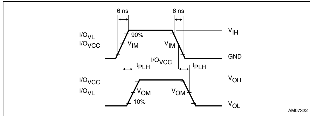
Figure 5. Waveform - propagation delay (f = 1 MHz, 50% duty cycle)
