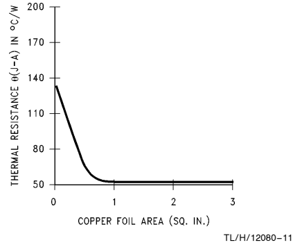
FIGURE 5. \theta_{(J-A)} vs Copper (2 ounce) Area for the SOT-223 Package
