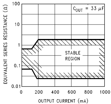
FIGURE 1. ESR Limits
