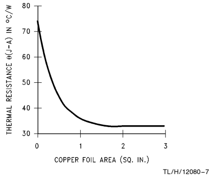
FIGURE 3. \theta_{(J-A)} vs Copper (1 ounce) Area for the TO-263 Package
