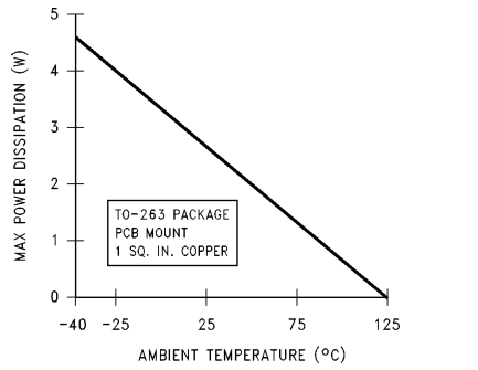
FIGURE 4. Maximum Power Dissipation vs T_{AMB} for the TO-263 Package
