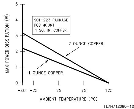
FIGURE 6. Maximum Power Dissipation vs T_{AMB} for the SOT-223 Package
