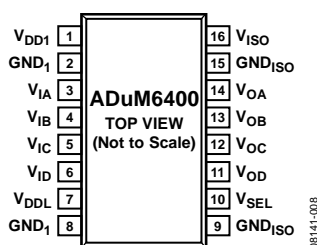
Figure 8. ADuM6400 Pin Configuration
