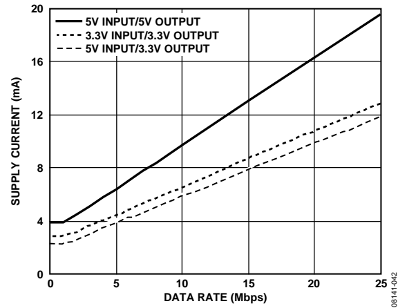
Figure 22. Typical I_{CHN} Supply Current per Reverse Data Channel (15 pF Output Load)
