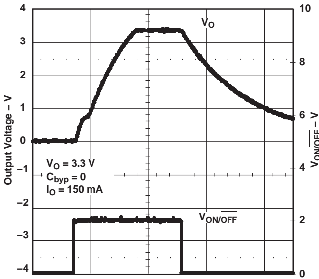
TURN-ON TIME
