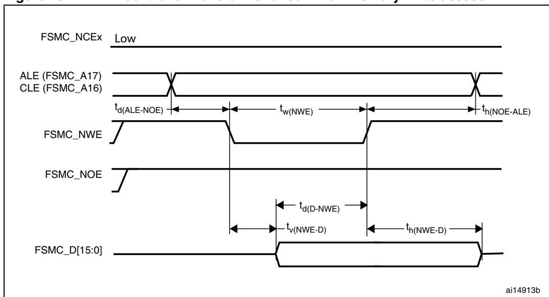
Figure 40. NAND controller waveforms for common memory write access
