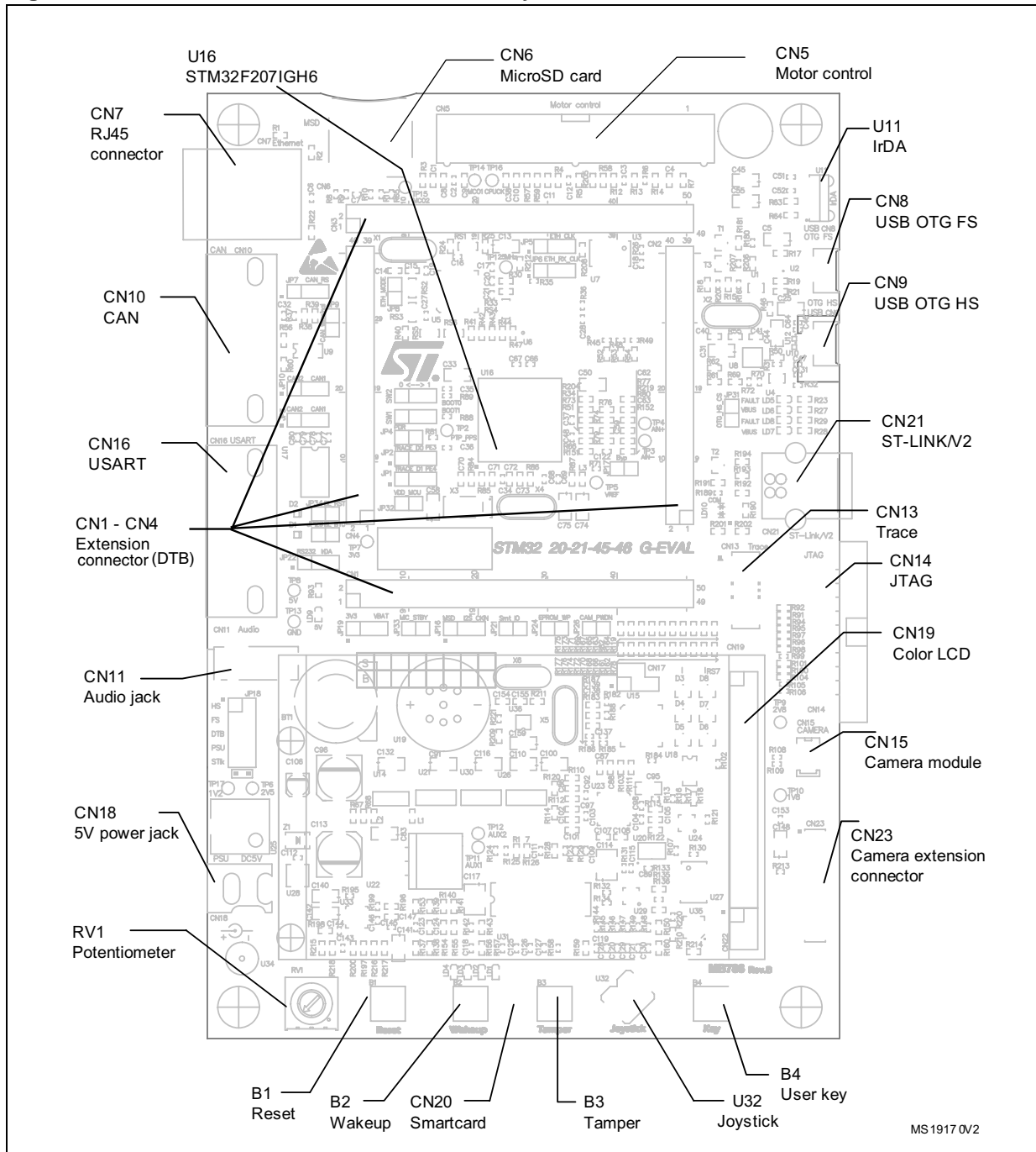
Figure 3. STM3221G-EVAL evaluation board layout
