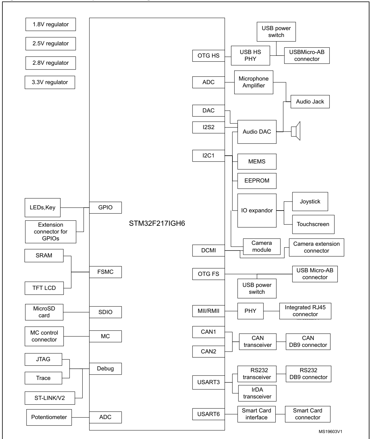
Figure 2. Hardware layout and configuration
