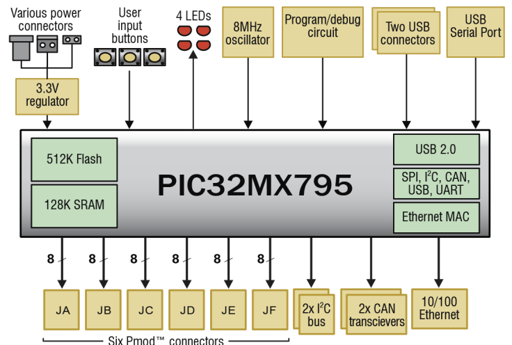
Cerebot MX7cK Circuit Diagram
