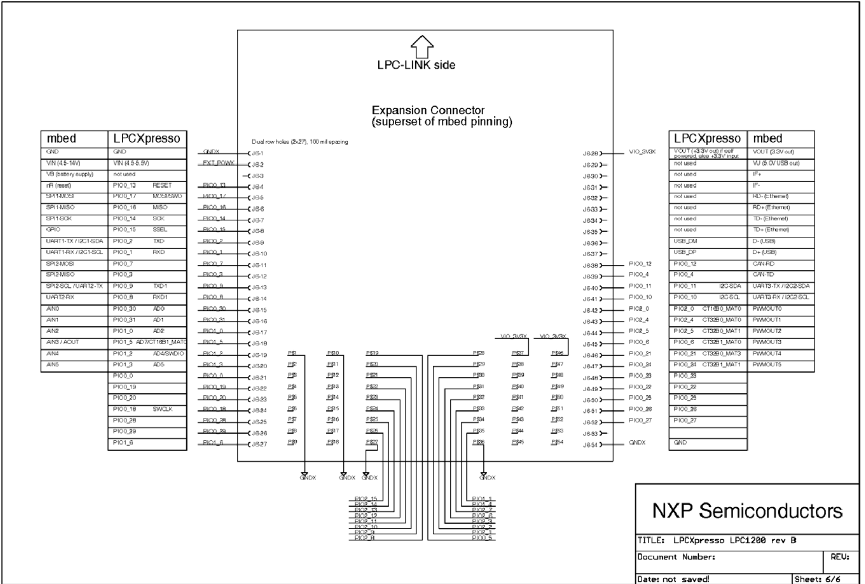
Fig 43. Schematic for the LPCXpresso LPC1200 target side, part 2
