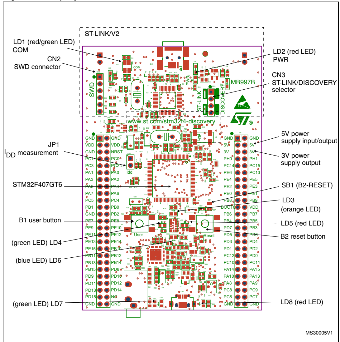
Figure 3. Top layout
