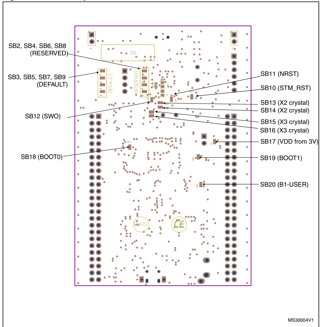
Figure 4. Bottom layout
