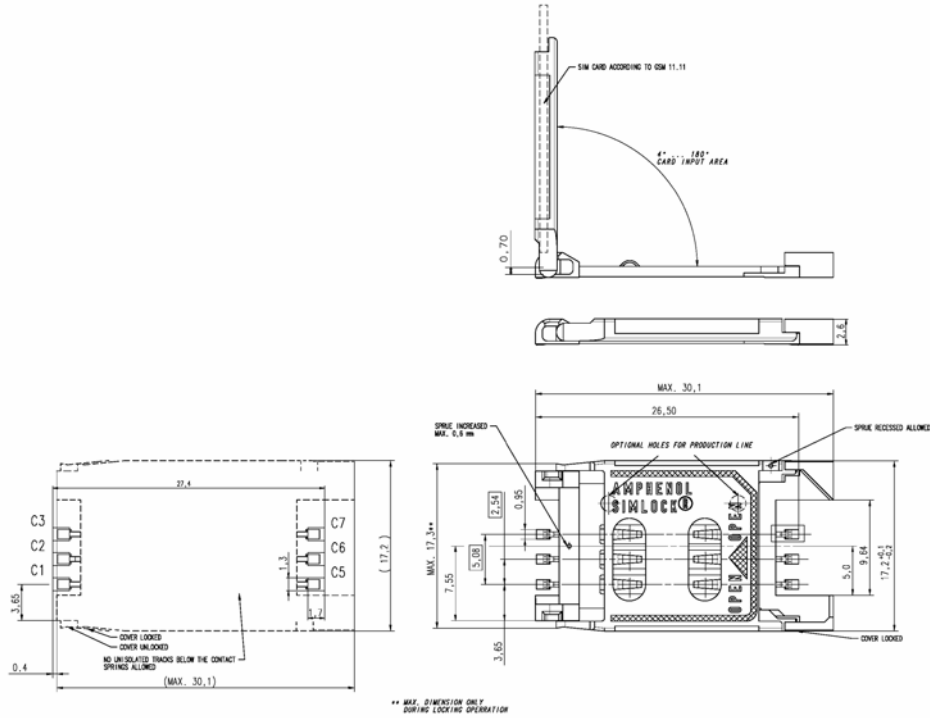
Figure 20: Amphenol C707-10M006 512 2 SIM card holder
