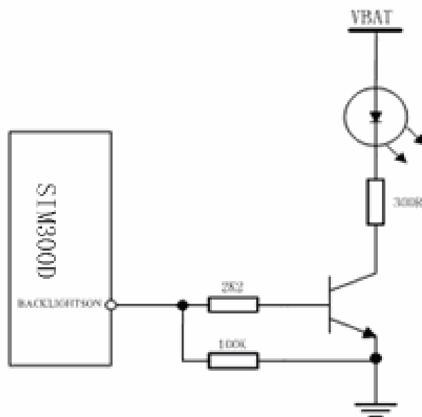
Figure 24: Reference circuit for Network status LED
