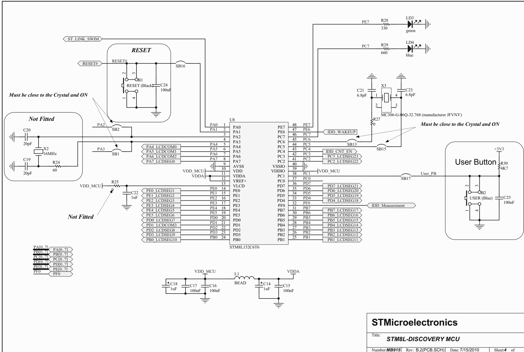
Figure 16. STM8L MCU
