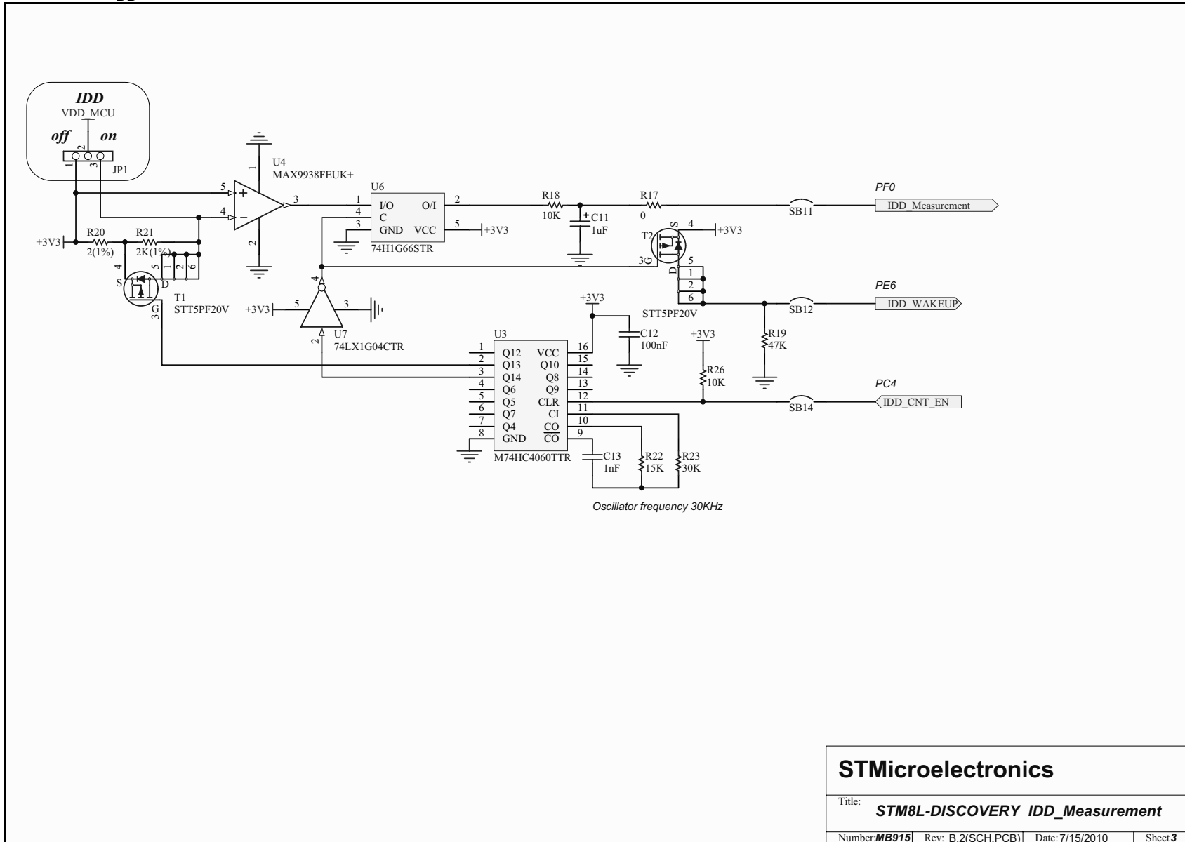
Figure 15. I_{DD} measurement
