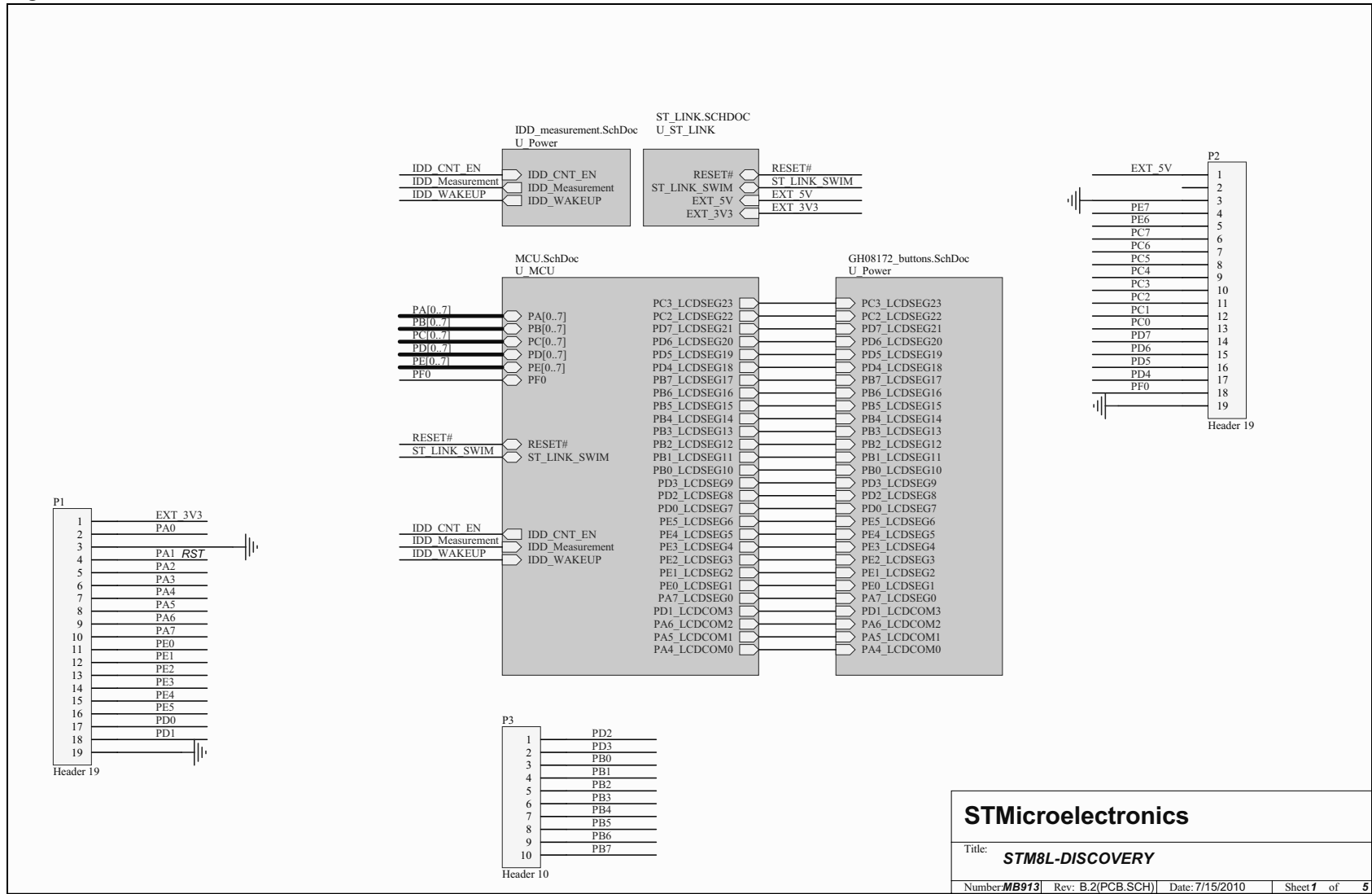
Figure 13. STM8L-DISCOVERY
