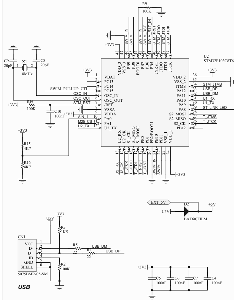
Figure 17. ST-Link (SWIM only)
