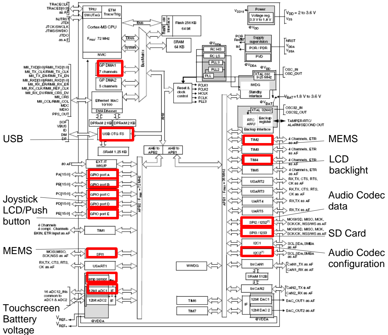
Illustration 5.1: STM32F107 peripherals
