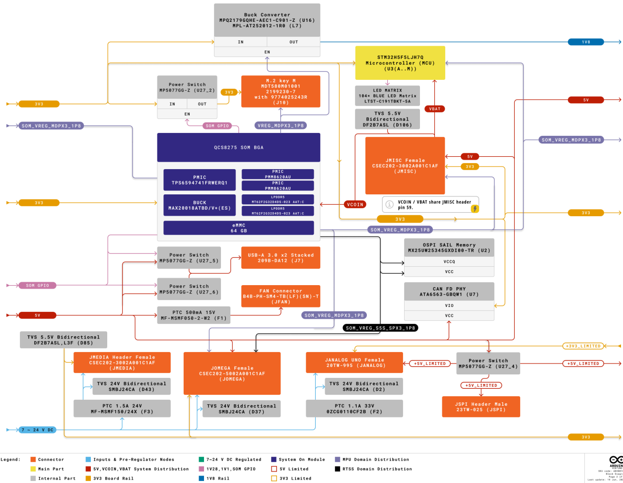
Arduino VENTUNO Q Power Tree (Page 2/3)
