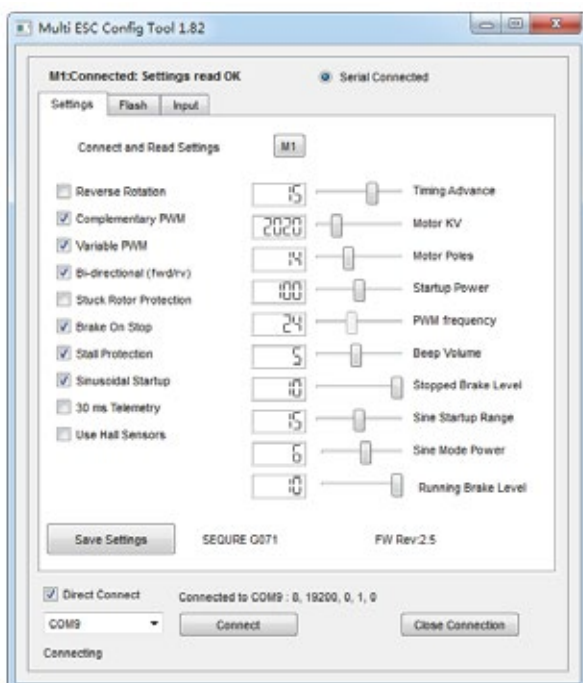
AM32 firmware visual programming parameter adjustment interface
