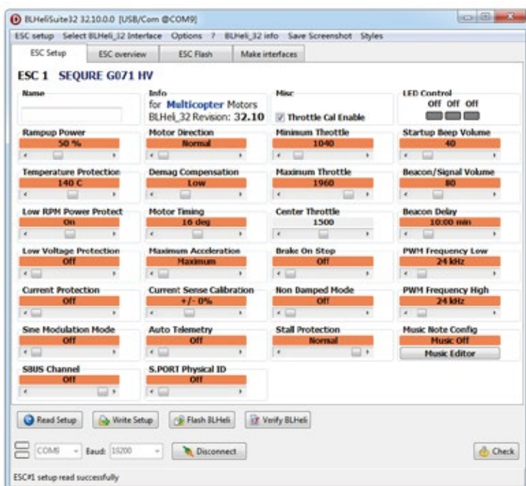
BLHeli_32 firmware visual programming parameter adjustment interface
