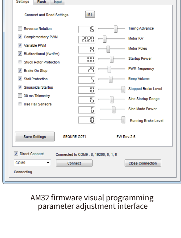
AM32 firmware visual programming parameter adjustment interface
