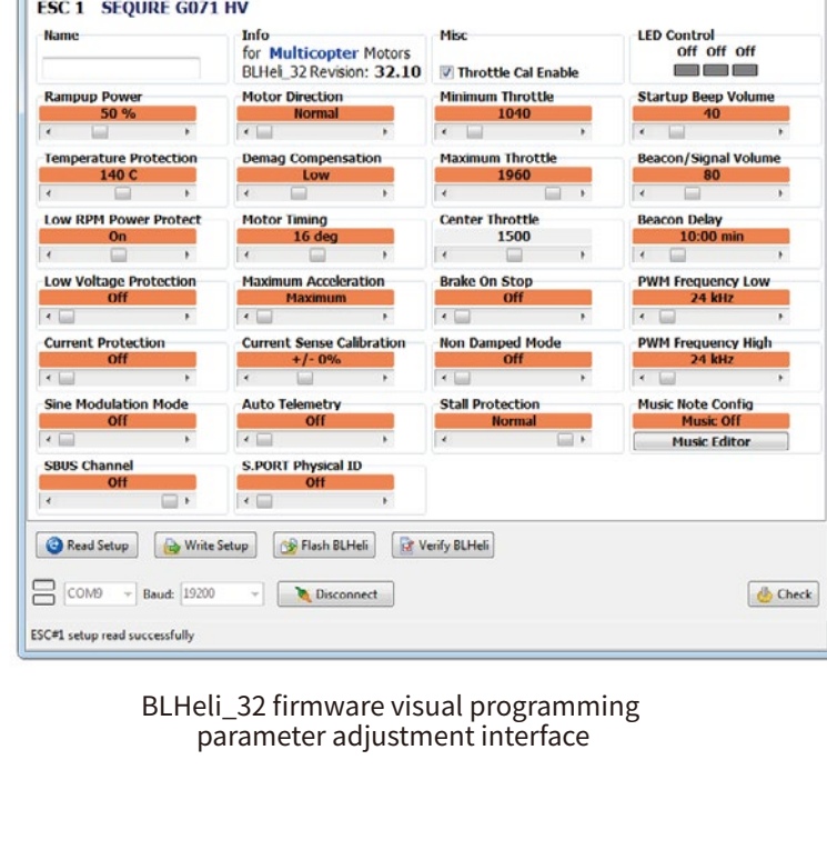
BLHeli_32 firmware visual programming parameter adjustment interface
