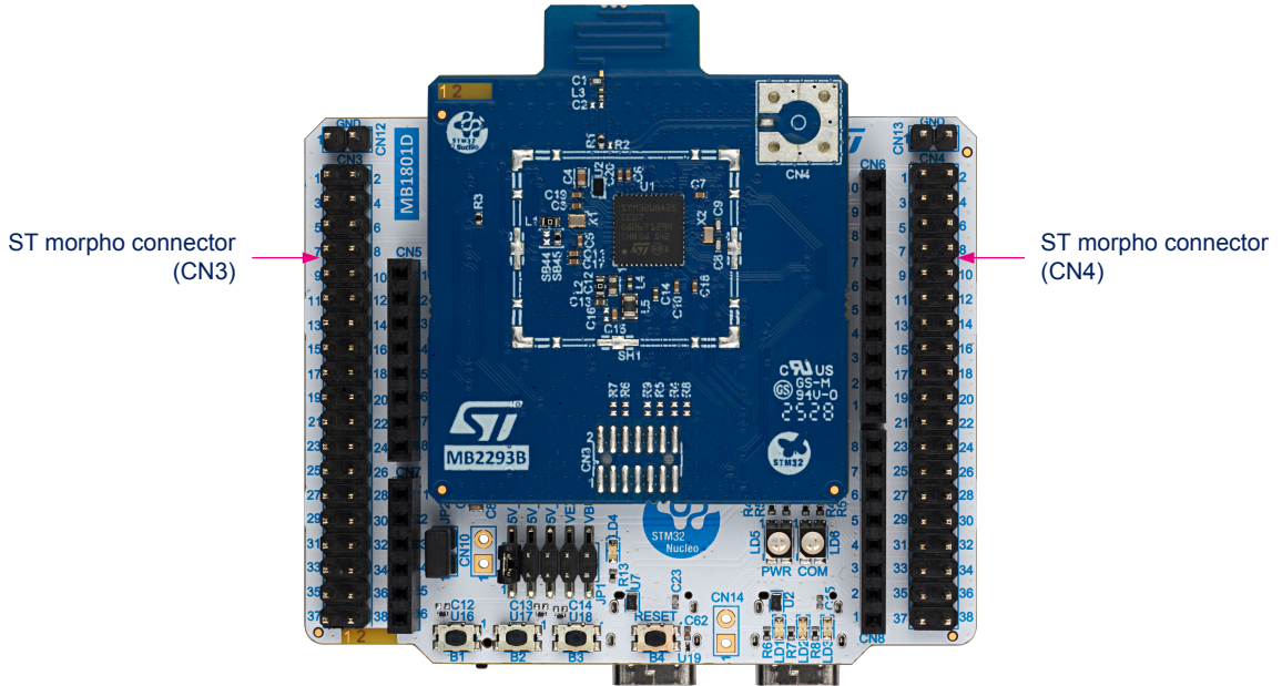
Figure 25. ST morpho connector location
