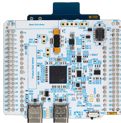
Figure 2. NUCLEO-WBA25CE1 bottom view
