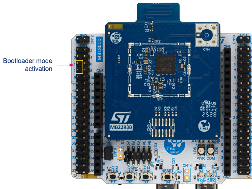
Figure 16. Bootloader activation
