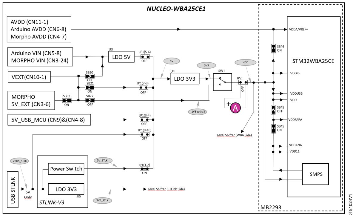
Figure 10. Current measurement with an ammeter
