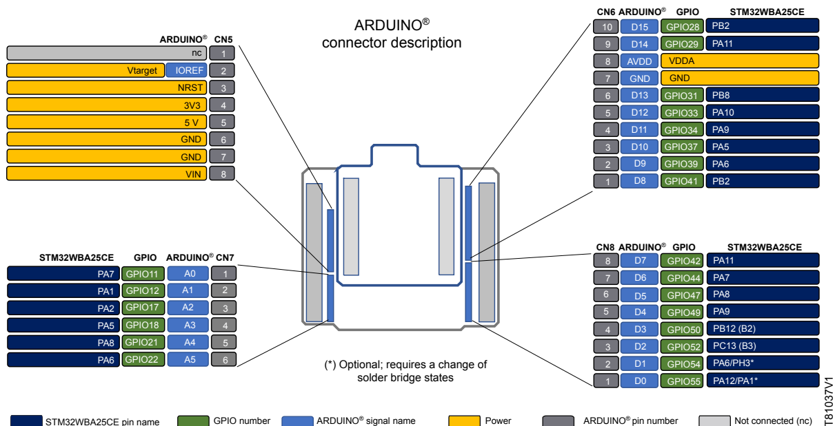
Figure 24. pinout
