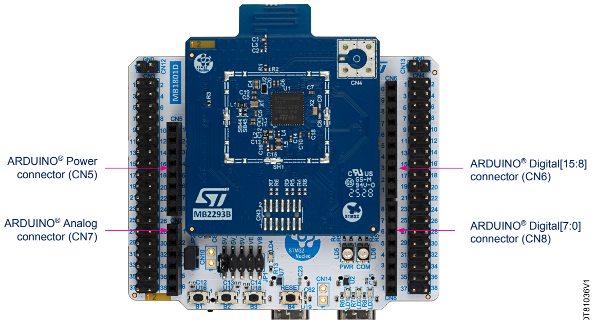
Figure 23. ARDUINO® Uno V3 connector location
