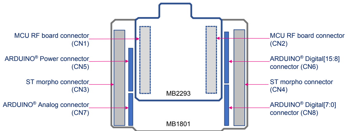
Figure 22. ARDUINO® Uno V3, ST morpho, and MCU RF board connector location
