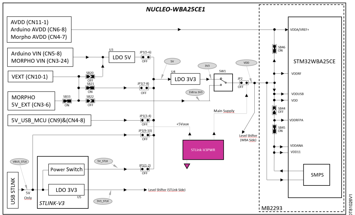
Figure 12. Current measurement with STLINK-V3PWR
