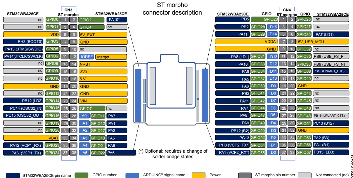
Figure 26. ST morpho pinout
