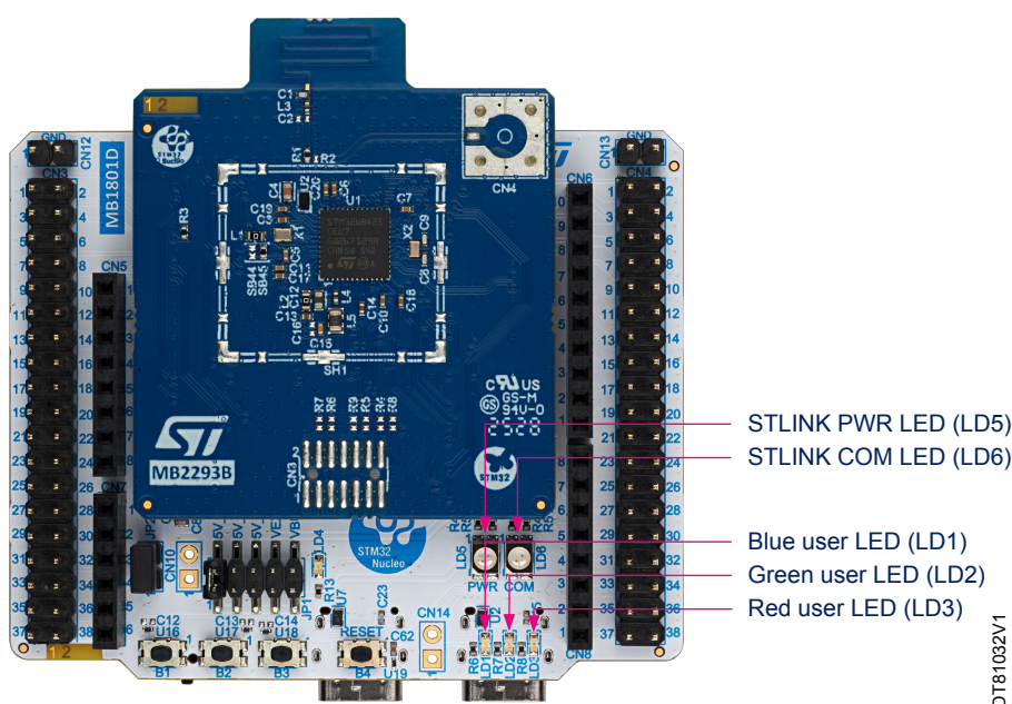
Figure 17. LEDs on NUCLEO-WBA25CE1
