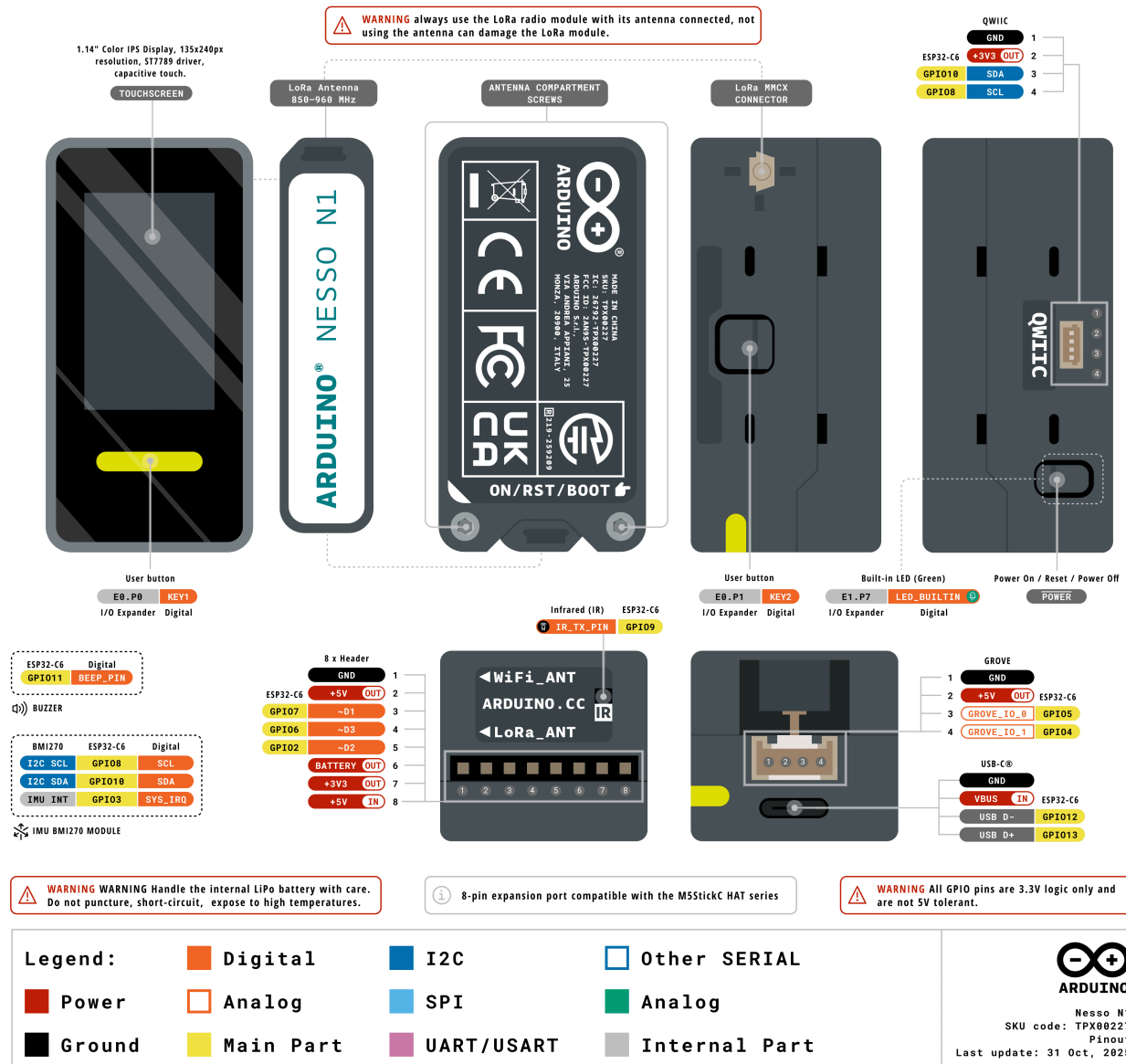
Nesso N1 Pinout - Simplified Version
