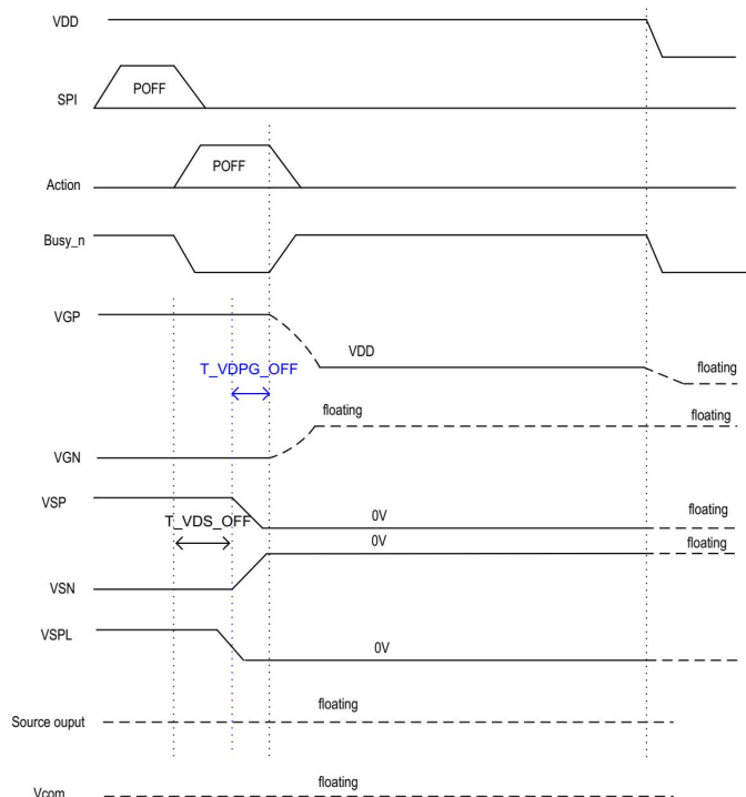
Power off Sequence(R02h=01)
