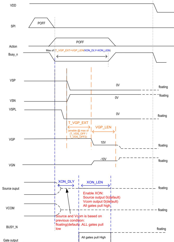
Power off Sequence(R02h=01)
