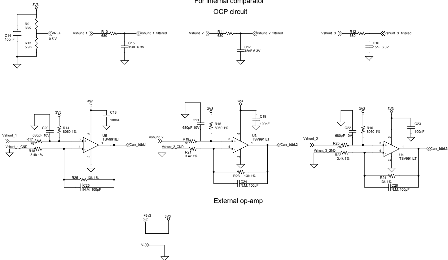
Figure 16. STEVAL-ESC001V1 circuit schematic (3 of 4)
