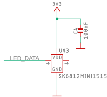
RGB LED
