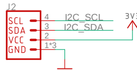
QW/ST connector
