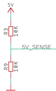
5V sense
