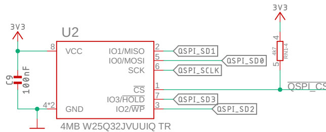
Flash memory
