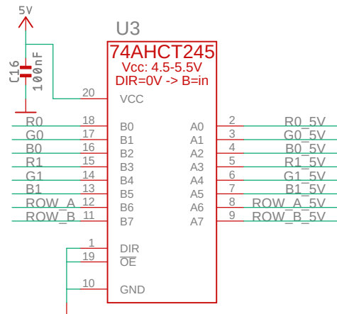
5V level shifters
