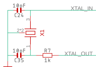
Crystal oscillator
