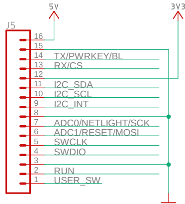
Expansion header
