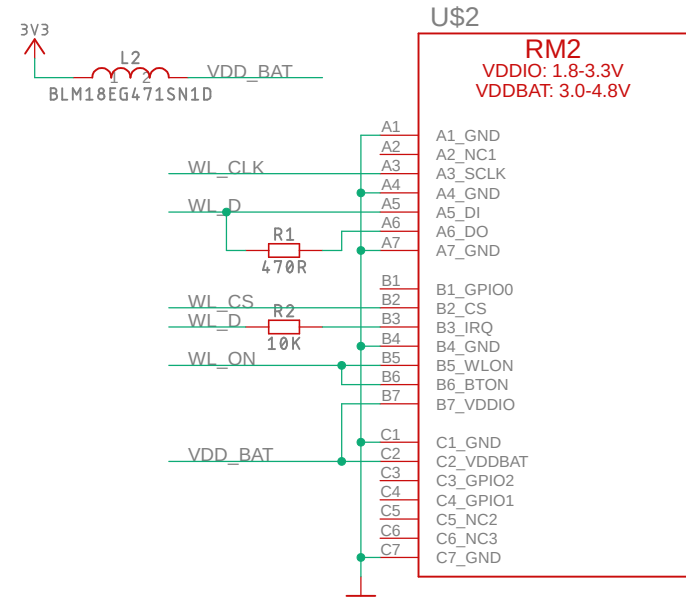
Wireless Module
