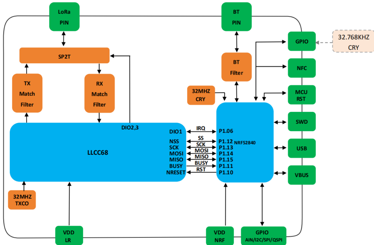
Figure 1:nRFLRCC68 Schematic diagram
