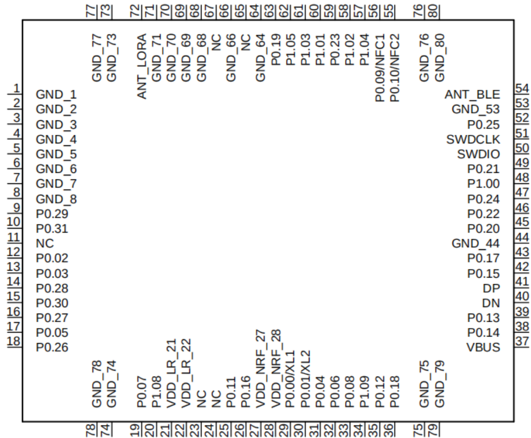
Figure 3:nRFLRCC68 Pin arrangement
