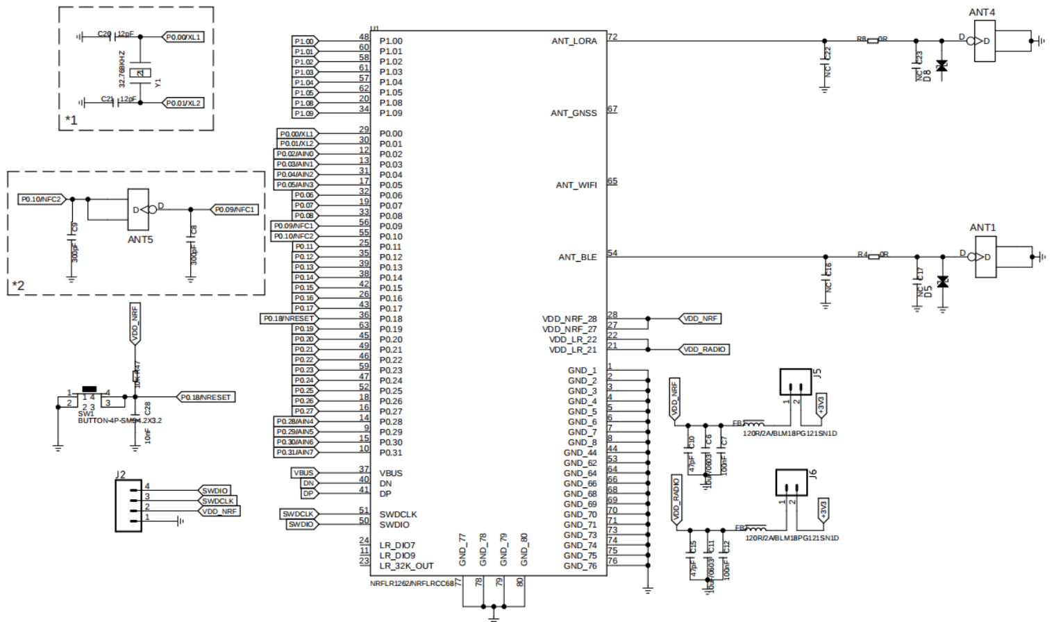
Figure 6:Reference design based on nRFLRCC68
