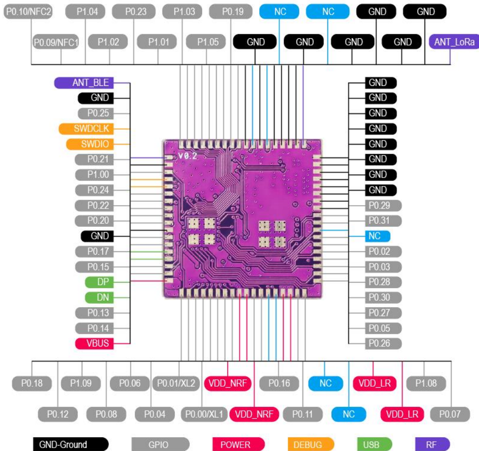
Figure 2:nRFLRCC68 Pin Definition
