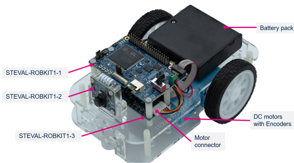
Figure 2. STEVAL-ROBKIT1 kit component placement
