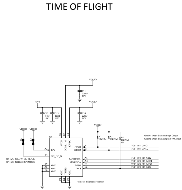
Figure 60. STEVAL-ROBKIT1-3 schematic (2 of 3)
