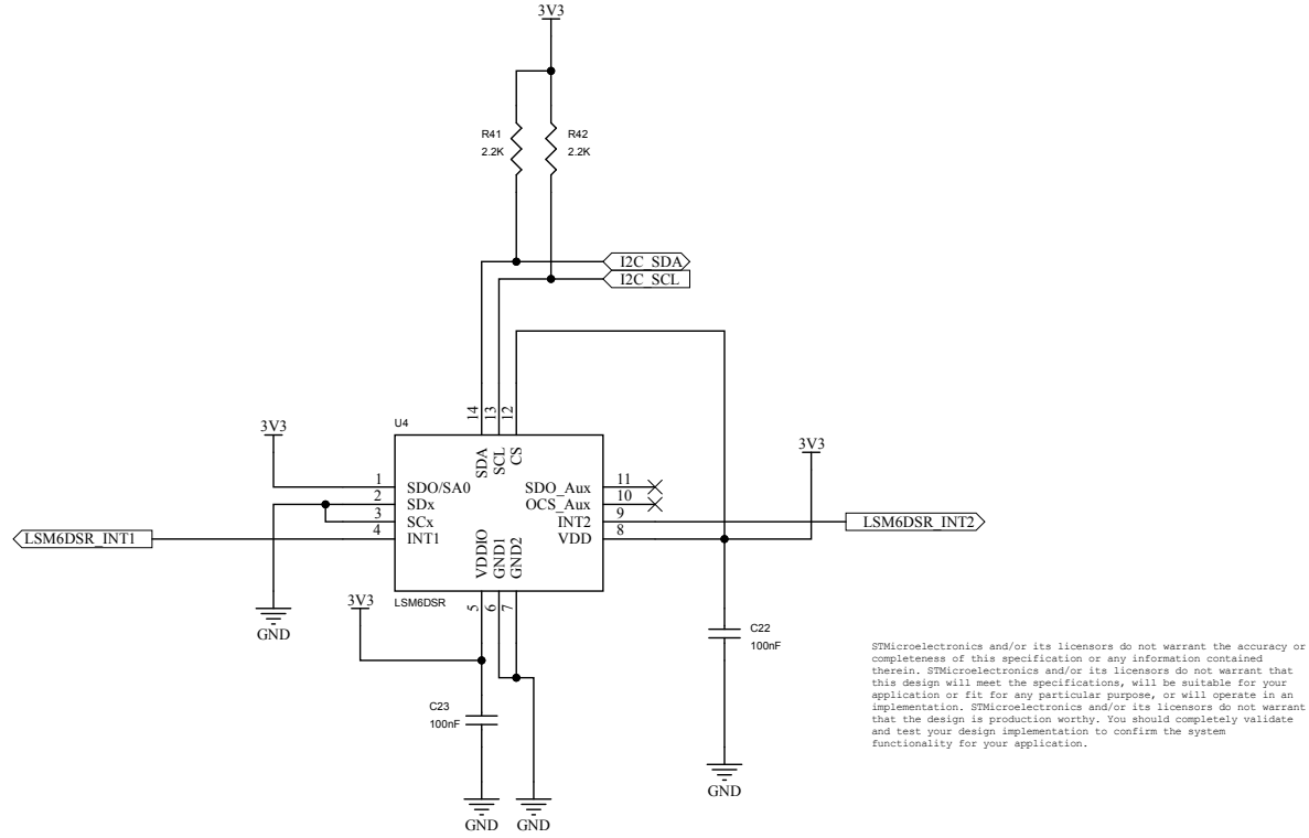
Figure 56. STEVAL-ROBKIT1-2 schematic (3 of 5)
