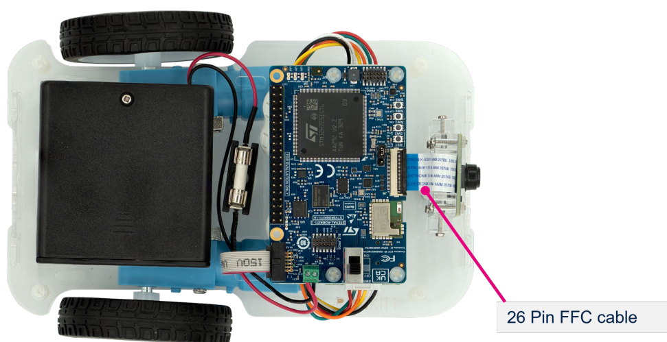
Figure 12. Connection of 26-pin FFC cable
