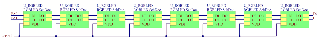
LED extension
