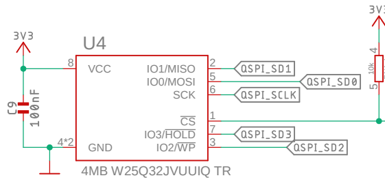
Flash memory
