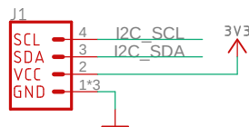
QW/ST connector
