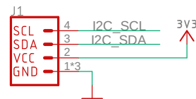
QW/ST connector
