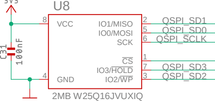
Flash memory
