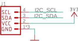
Qw/ST connector
