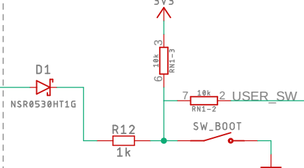
Combined USB boot & user switch
