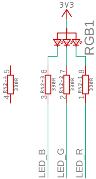
RGB LED
