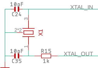
Crystal oscillator
