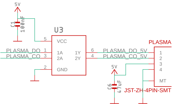
Plasma smart LED output with level shifting
