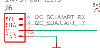
QW/ST connector
