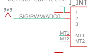
QW/ST connector
