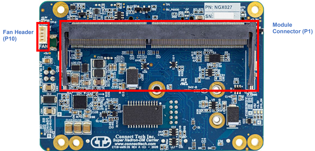
Bottom View
