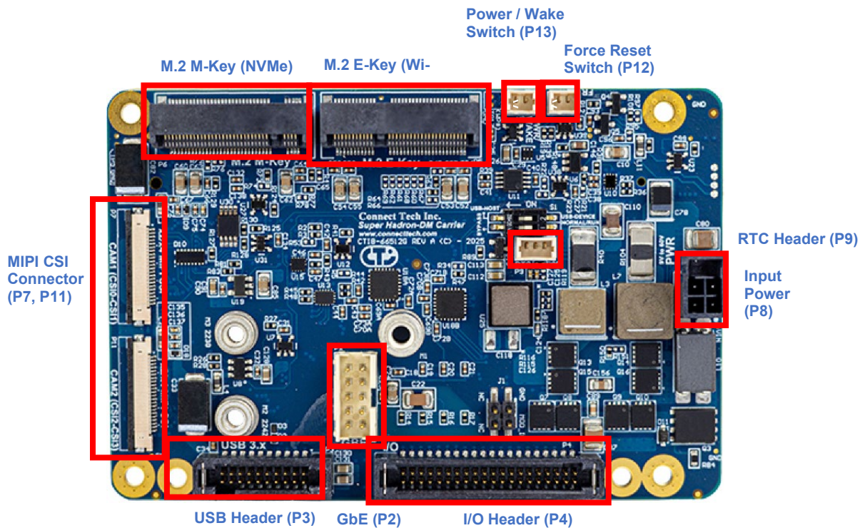
Bottom View
