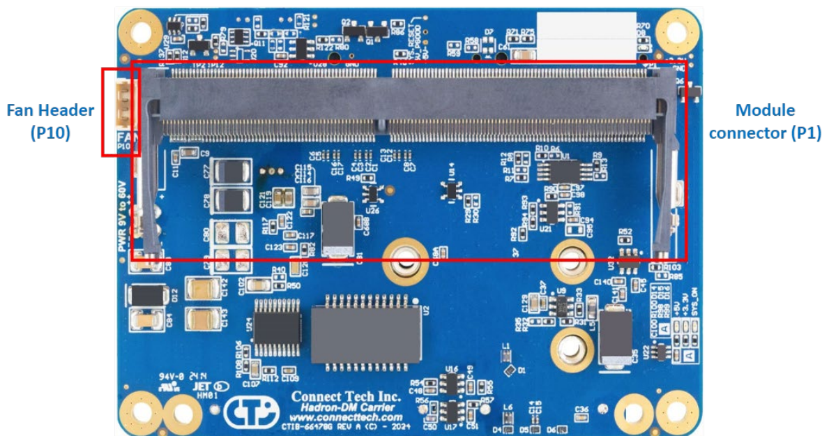
Bottom View
