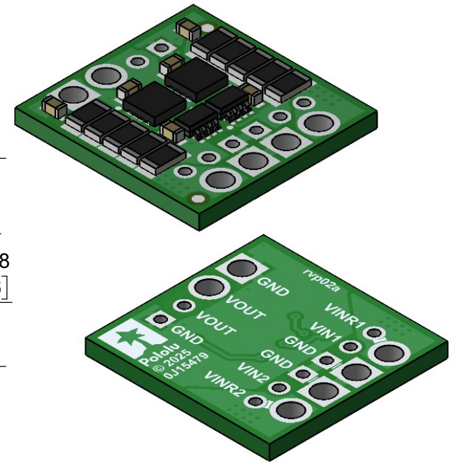
③ Isometric view Scale 2:1
