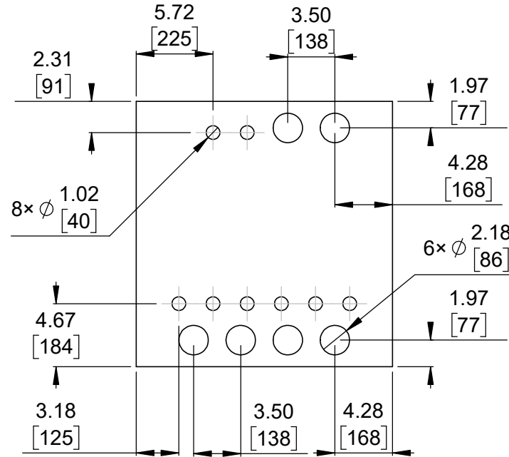
② Connector callouts (bottom view) Scale 5:2
