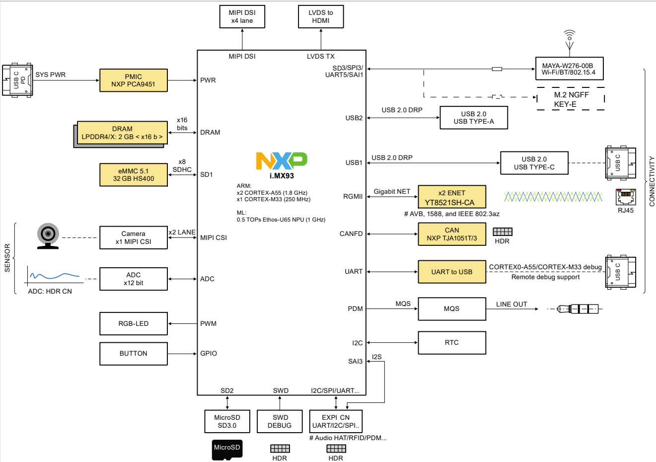
Figure 1. FRDM-IMX93 block diagram
