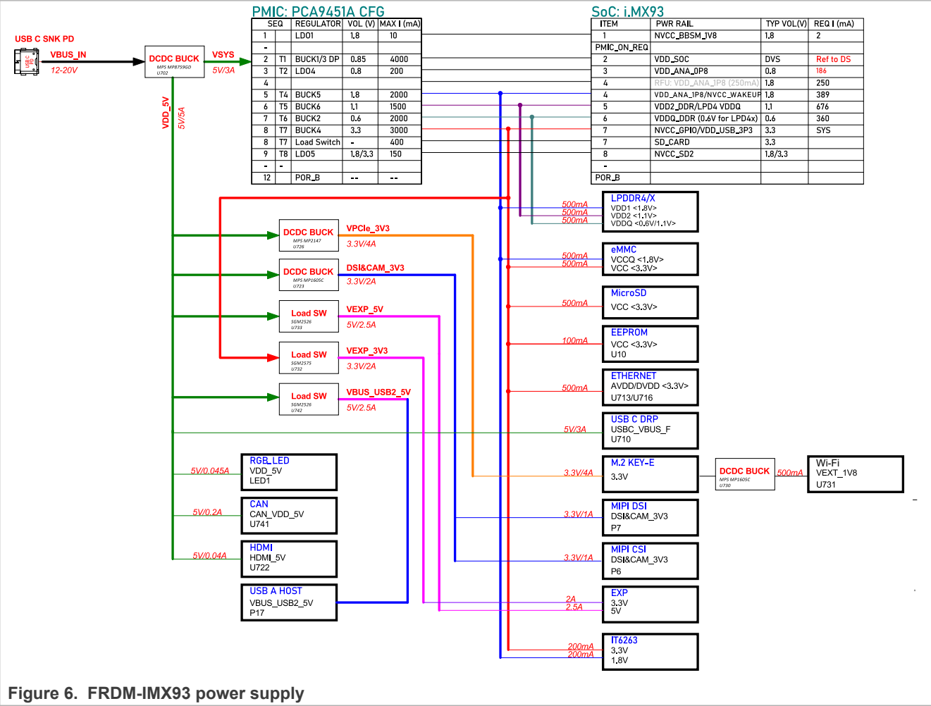
Figure 6 shows the FRDM-IMX93 power supply block diagram.
