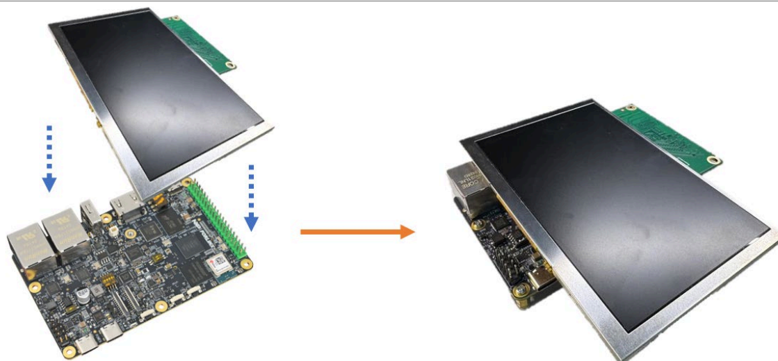
Figure 15. 5-inch Tianma LCD connection with FRDM-IMX93 through 40-pin connector
