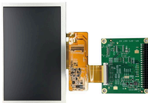
Figure 14. FPC connection between 5-inch Tianma LCD panel and adapter board
