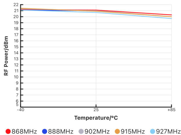
Figure 4 Max RF Power VS Temperature (868~927MHz)
