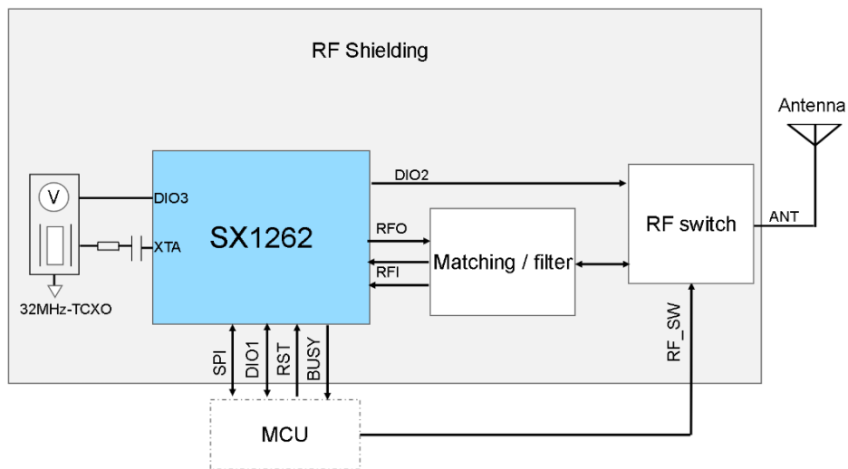
Figure 1 Wio-SX1262 Schematic Diagram
