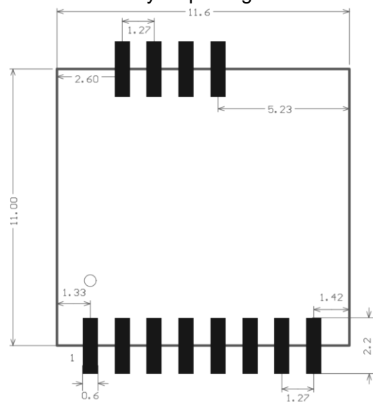
Figure 9 PCB Footprint
