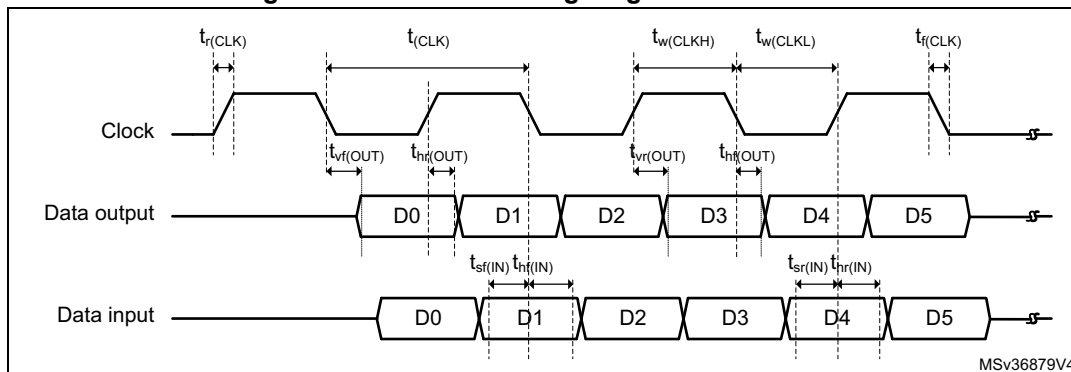
Figure 48. OCTOSPI timing diagram - DTR mode
