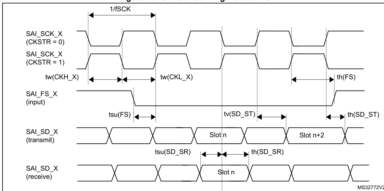
Figure 70. SAI slave timing waveforms
